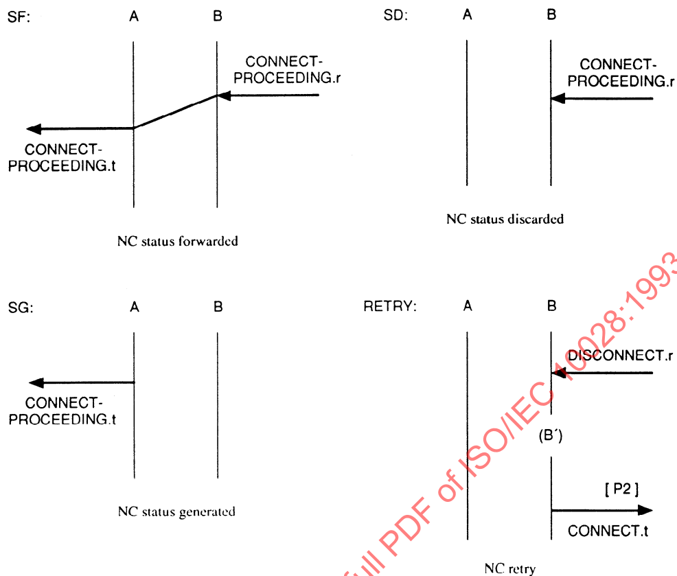
Figure 5 — NC establishment, NC proceeding subphase
