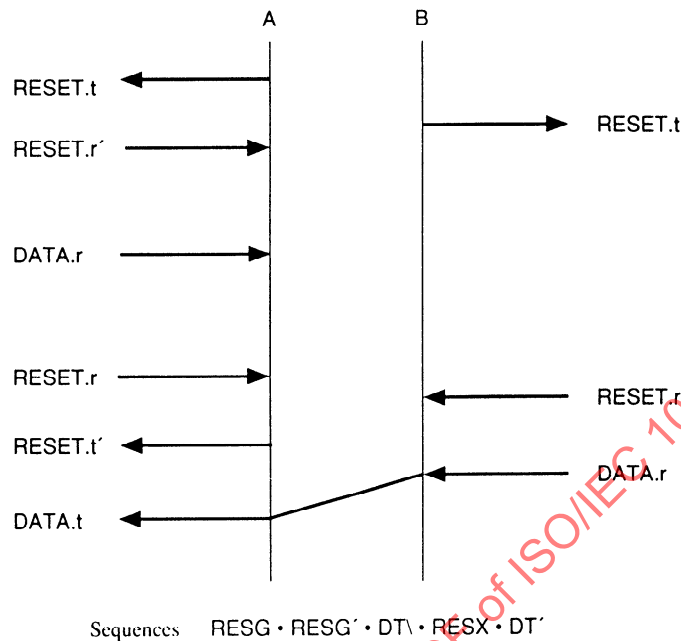
Figure 14 — Multiple resets in one reset subphase
