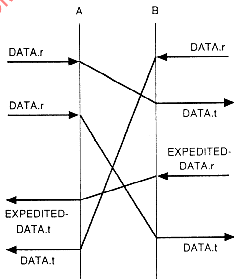
Figure 12 — Example of multiple combination methods
