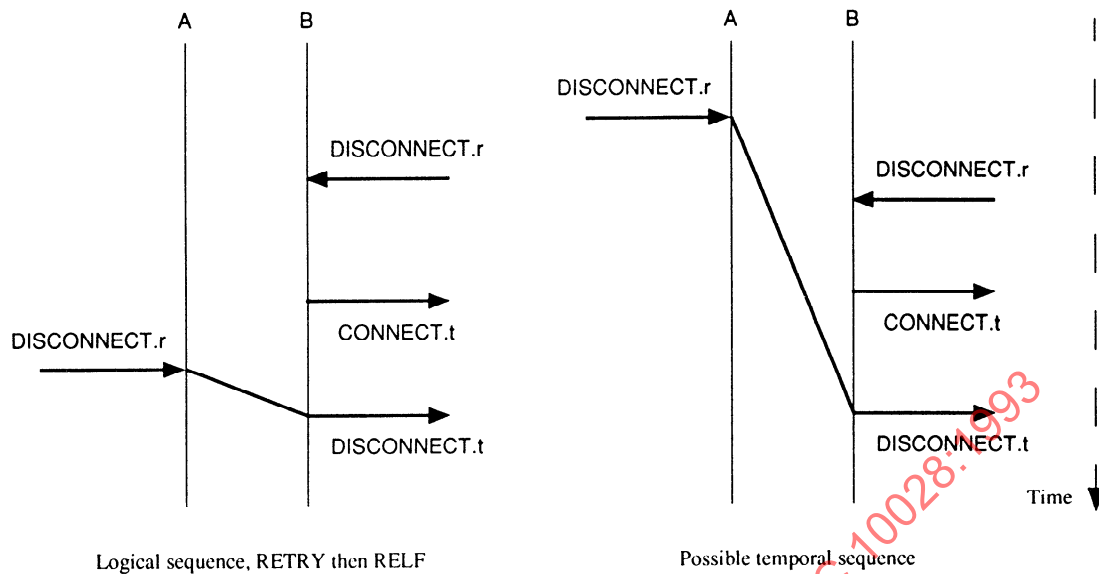
Figure 10 — Example of succession of elementary sequences
