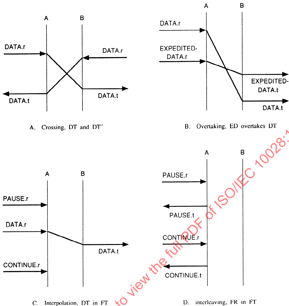
Figure 11 — Non-successive combinations of elementary sequences
