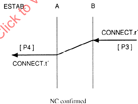
Figure 6 — NC establishment, NC confirmation subphase
