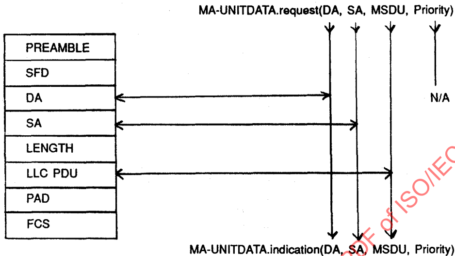
Figure A.1 - Mapping of MAC Service primitives to/from ISO/IEC 8802-3 MAC frames
