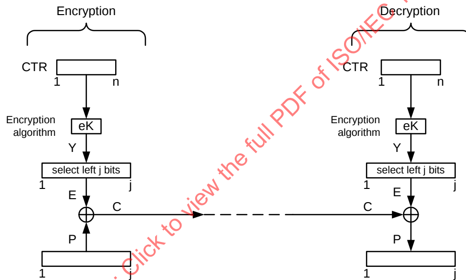
Figure C.5 – The Counter (CTR) mode of operation
