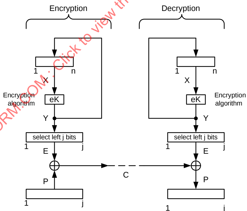
Figure C.4 – The Output Feedback (OFB) mode of operation
