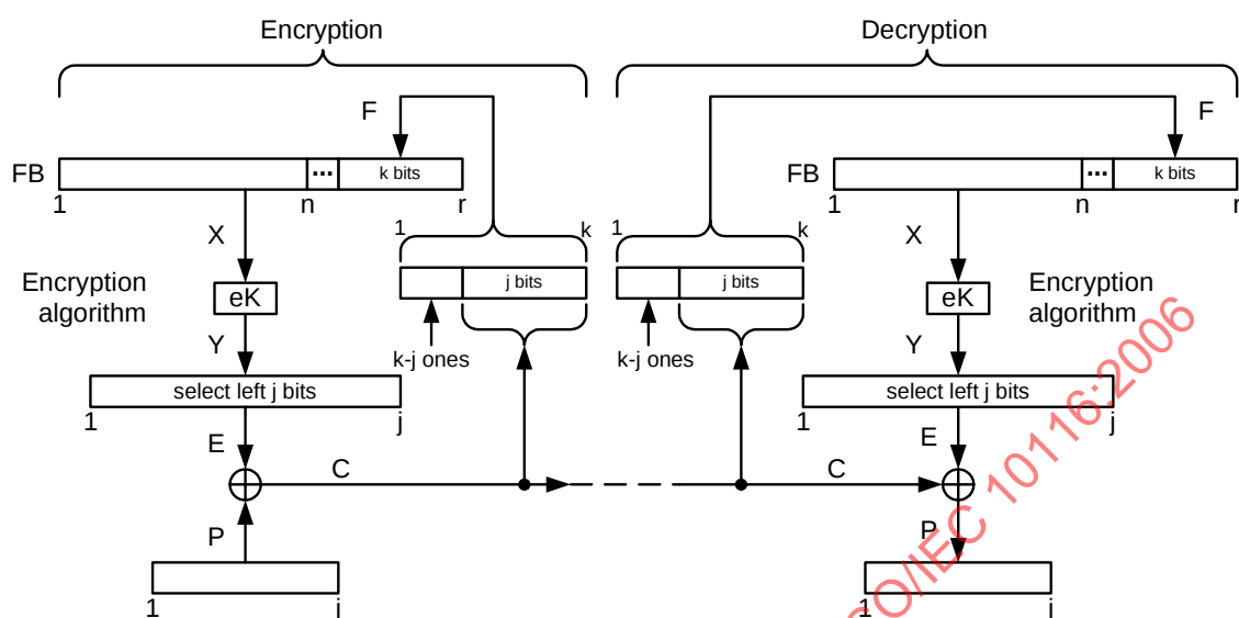
Figure C.3 – The Cipher Feedback (CFB) mode of operation
