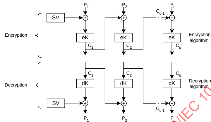
Figure C.1 – The Cipher Block Chaining (CBC) mode of operation with m = 1
