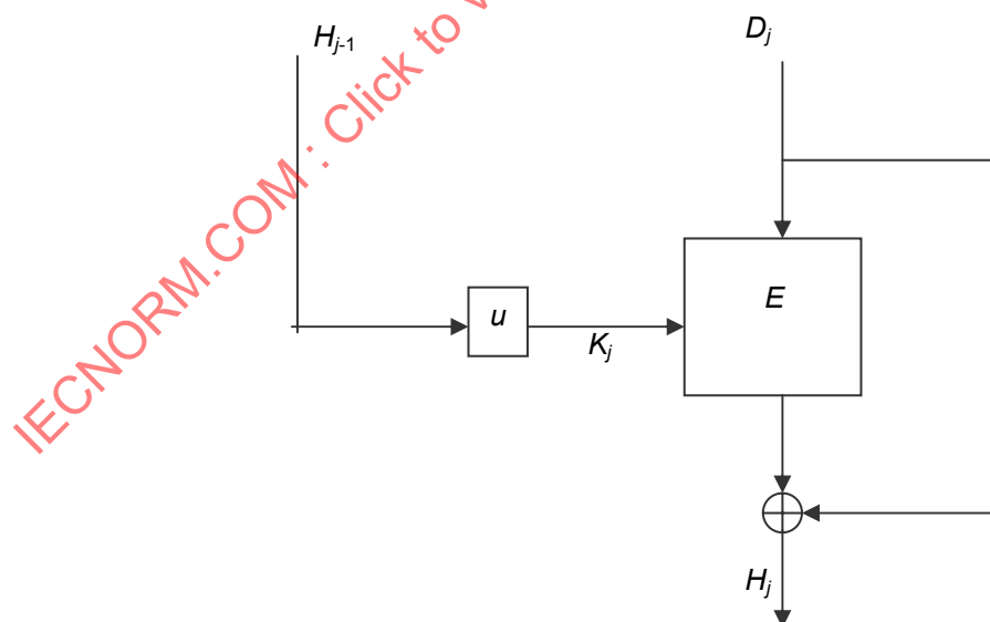
Figure 1 — Round function of hash-function 1
