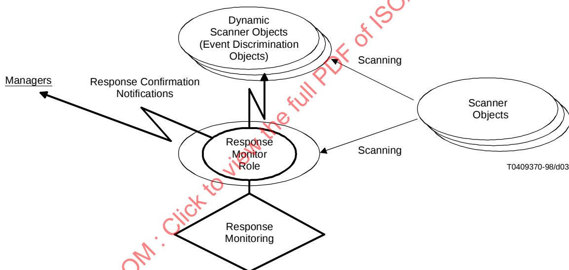
Figure 3 – Relationship between response monitor and scanner objects
