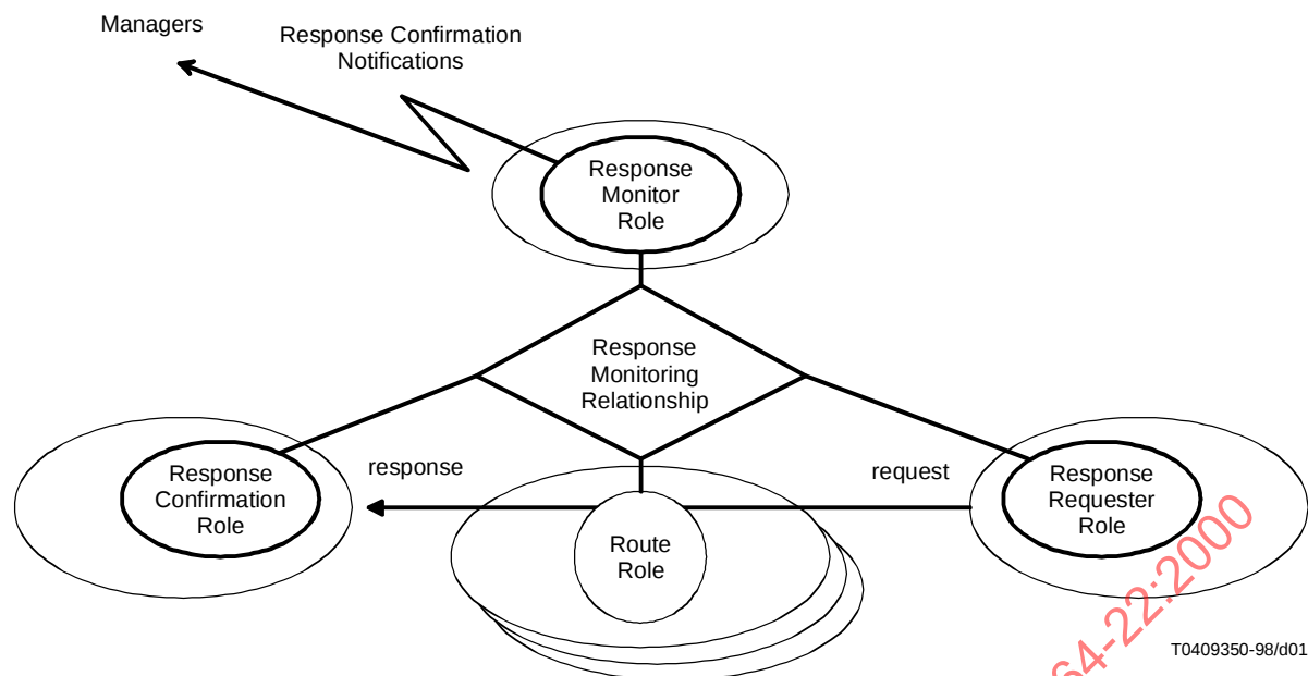
Figure 1 – Response Monitoring Model
