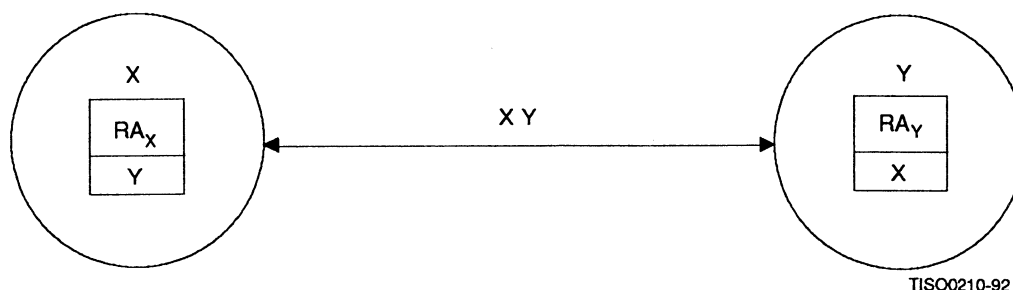
Figure 3 – Reciprocal relationship
