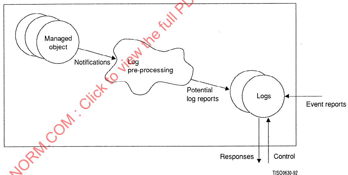
Figure 1 – Log management model
