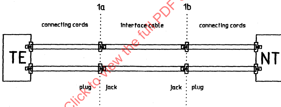
Figure B.1 — Cabling and connector arrangements
