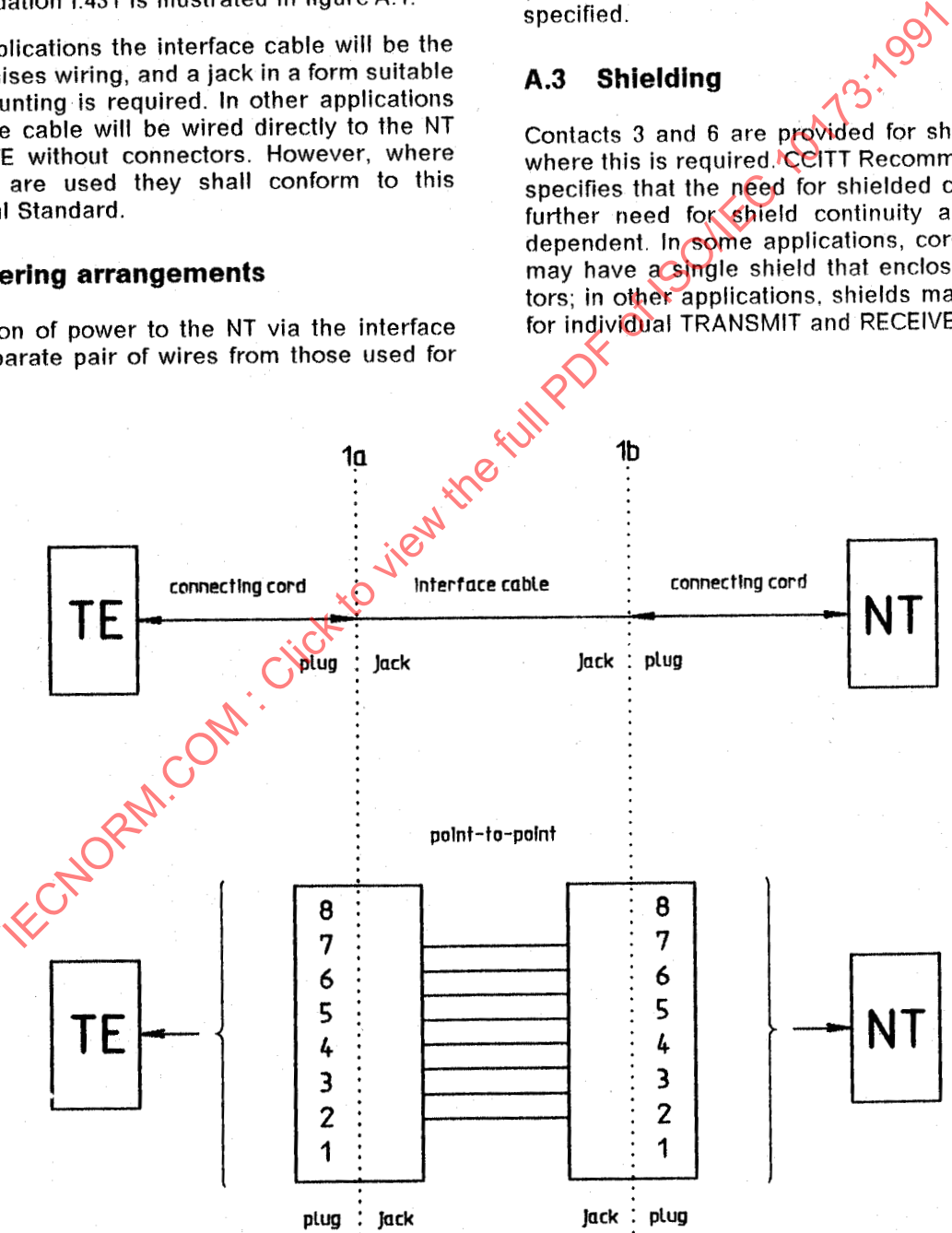
Figure A.1 — Cabling and connector arrangements
