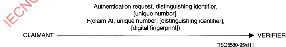
Figure 11 – Sub-class 3 – Unique number mechanism
