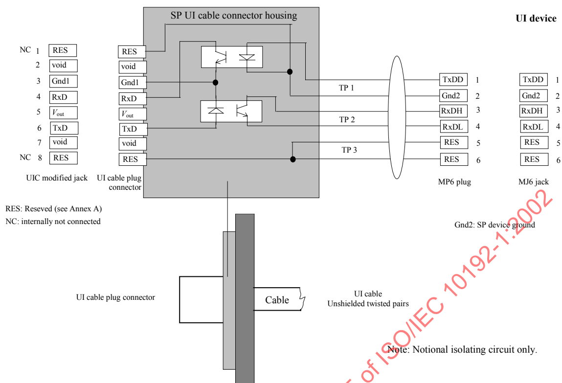
Figure 4 – SP UI cable
