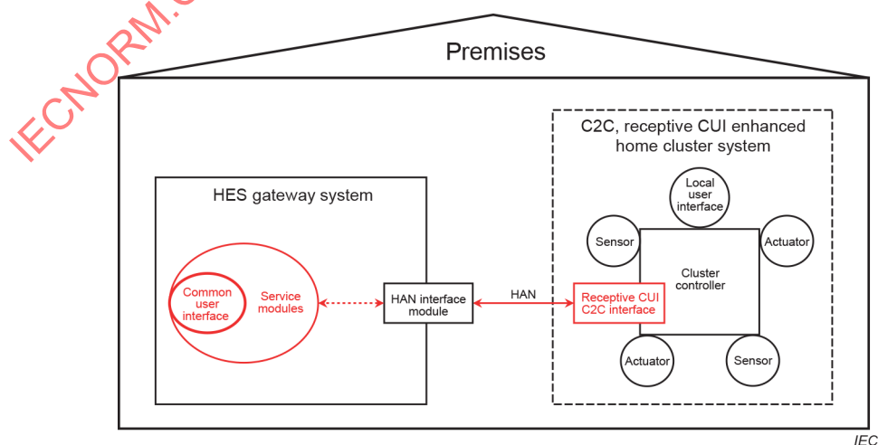
Figure 5 – CUI components of alternative #3: common user interface in a service module
