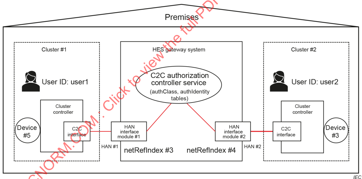
Figure 11 – Configuration of user identities and devices
