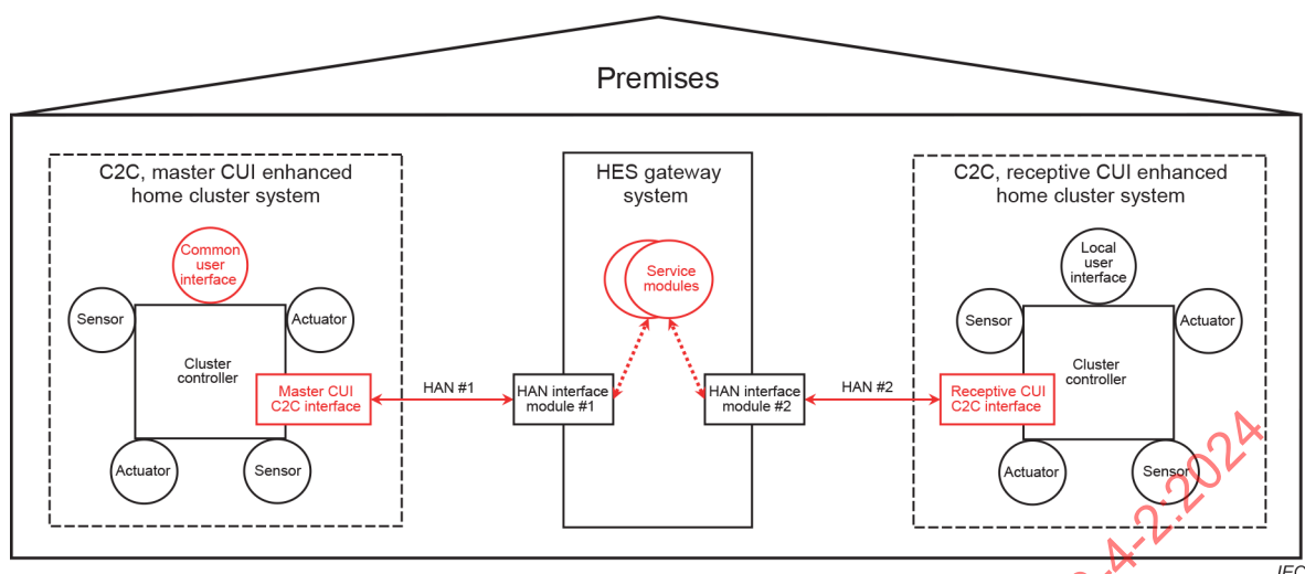
Figure 3 – CUI components of alternative #1: common user interface in a cluster
