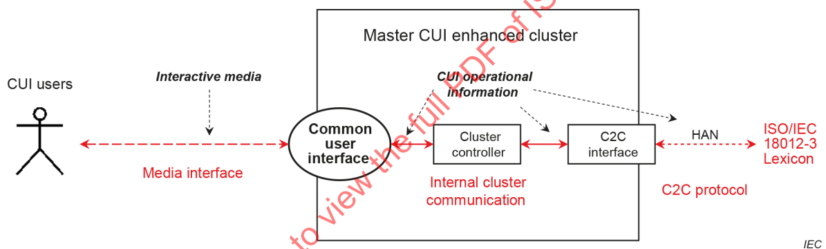
Figure 6 – Translation between CUI operational information and interactive media
