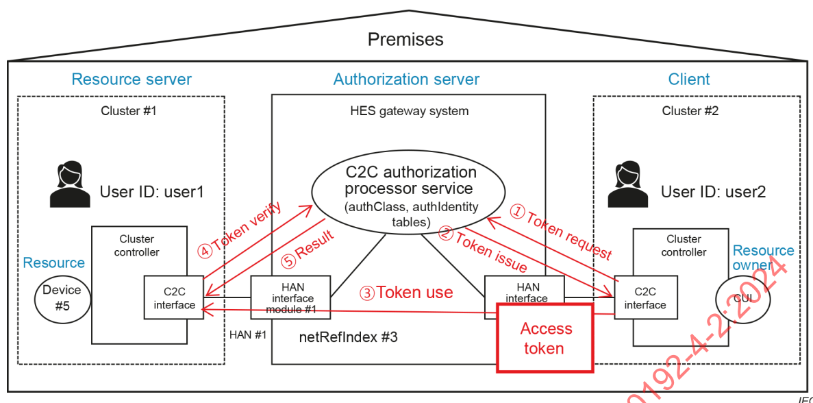
Figure 13 – C2C authorization procedure
