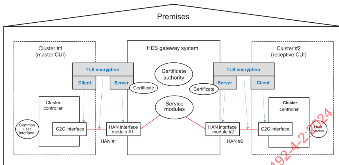
Figure 10 – TLS based C2C secure connection
