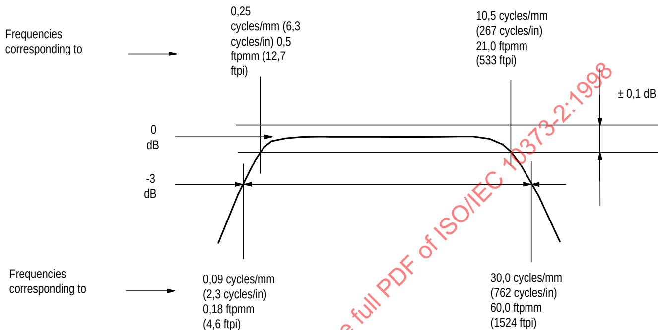
Figure 15 — Filter characteristic
