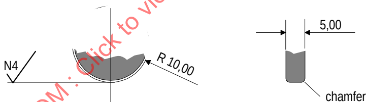
Figure 10 — Dimensions of the contact area of the dummy head
