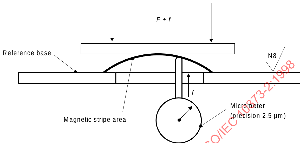
Figure 1 — Measuring arrangement
