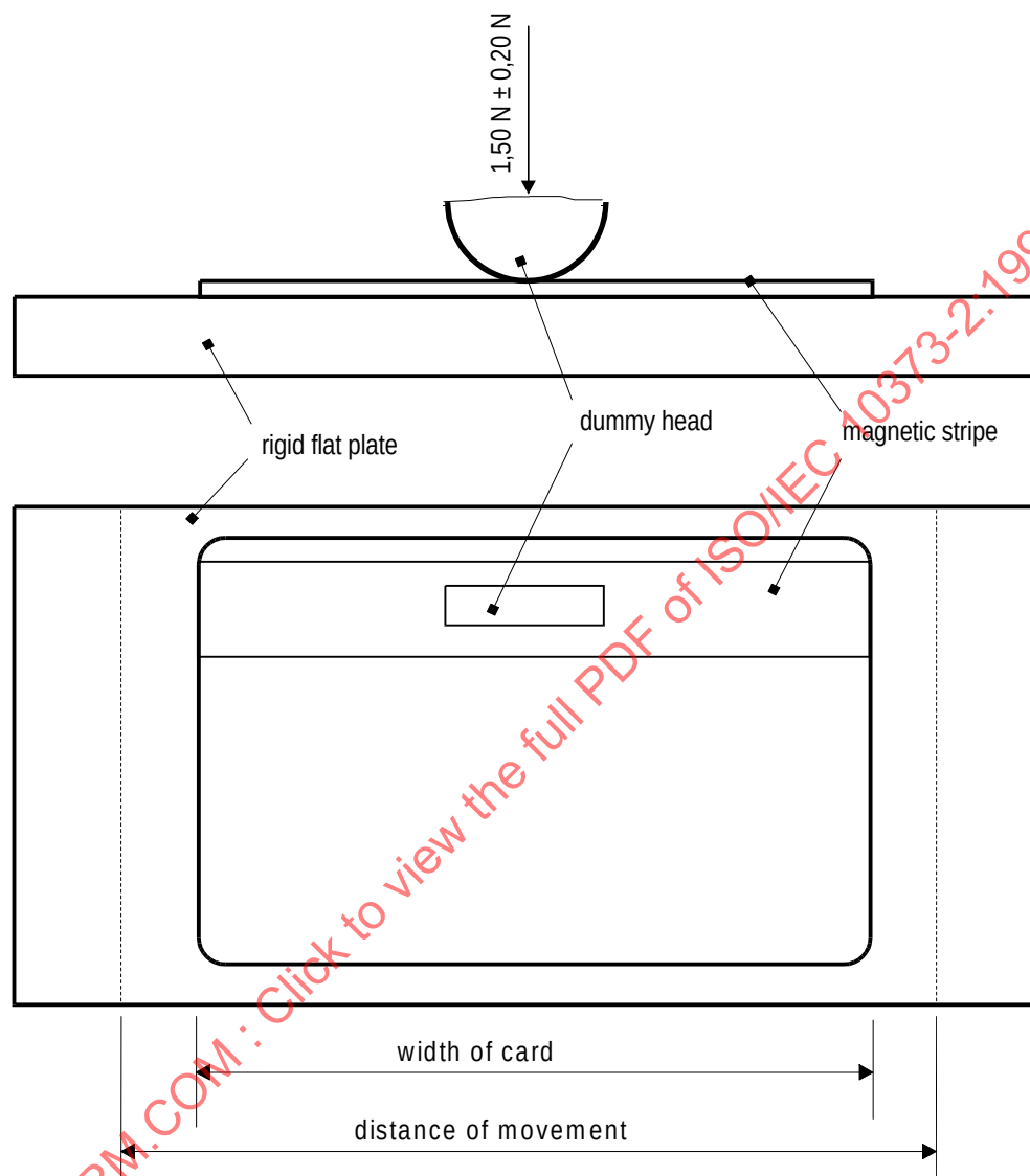
Figure 11 — Dummy head and magnetic stripe
