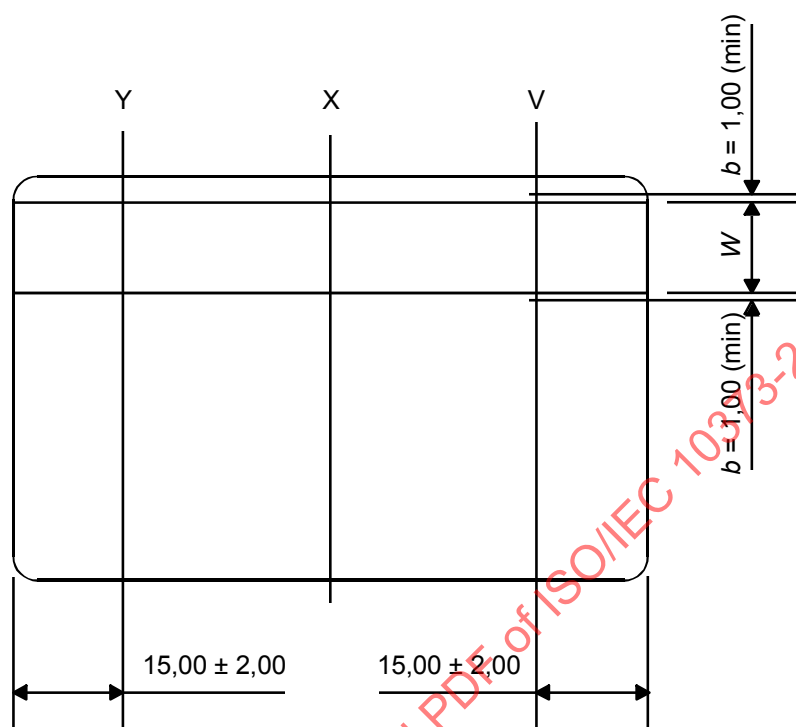
Figure 5 — Magnetic stripe profile measurement location
