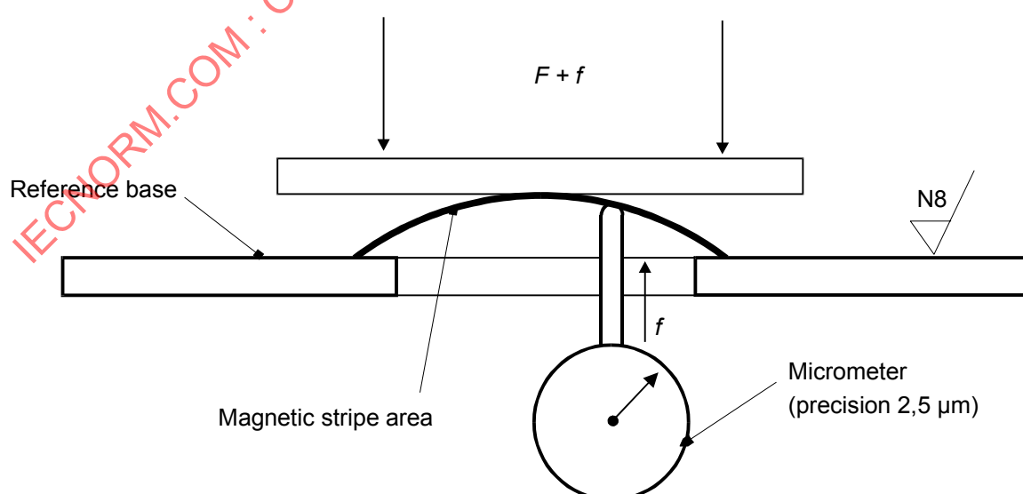
Figure 1 — Measuring arrangement
