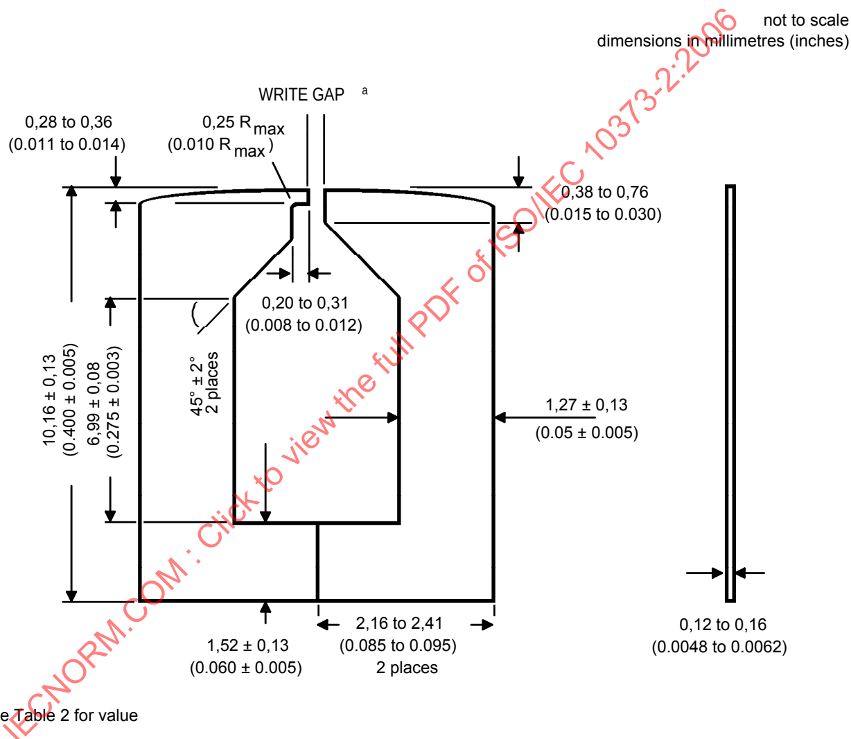
Figure 12 — Test write head laminations
