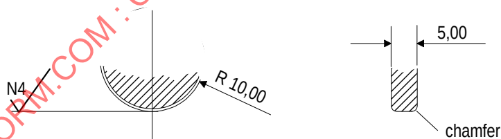
Figure 10 — Dimensions of the contact area of the dummy head
