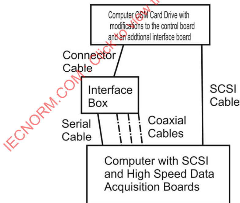
Figure 4 — Card tester (PMT) block diagram
