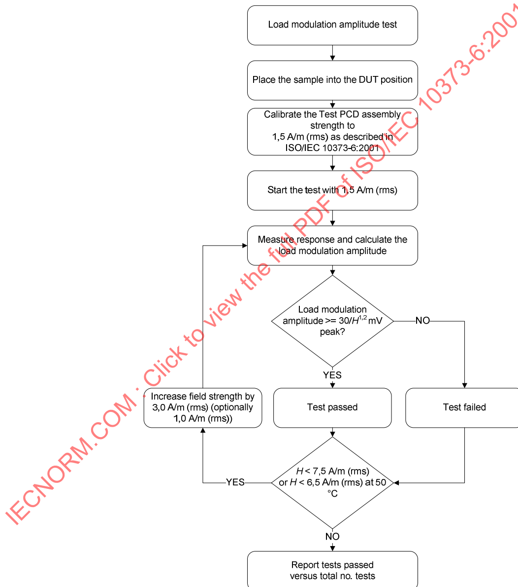
Figure L.1 — Test procedure for the load modulation amplitude test
