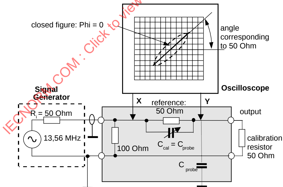
Figure B.1 — Calibration set-up (Step 1)
