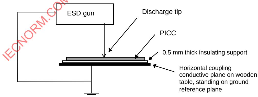
Figure 1 — ESD test circuit
