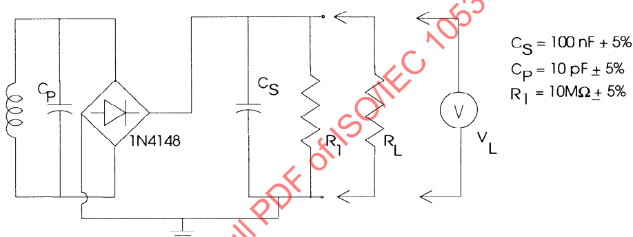
Figure A.1 - Magnetic Field Test Circuit
