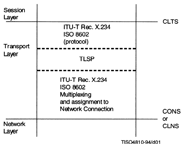
Figure 1 – TLSP with ITU-T Rec. X.234 | ISO 8602
