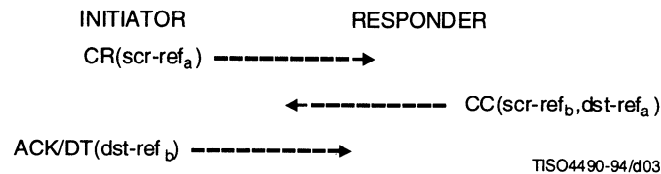
Figure 3 – Illustration of exchanges to support peer entity authentication
