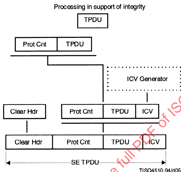
Figure 5 – TLSP Encapsulation Methods (TLSP's method for encapsulation and ICV generation in support of integrity as indicated in 6.3)
