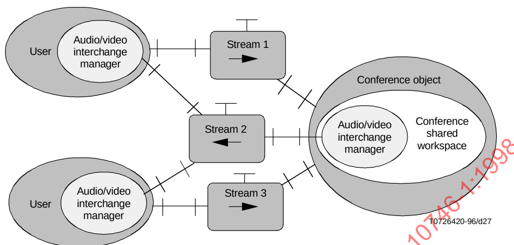
Figure 27 – MMCS configuration of objects involved in audio/video interchange
