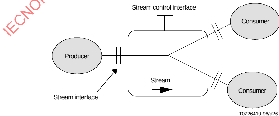
Figure 26 – Representation of an explicit binding (e.g. stream)
