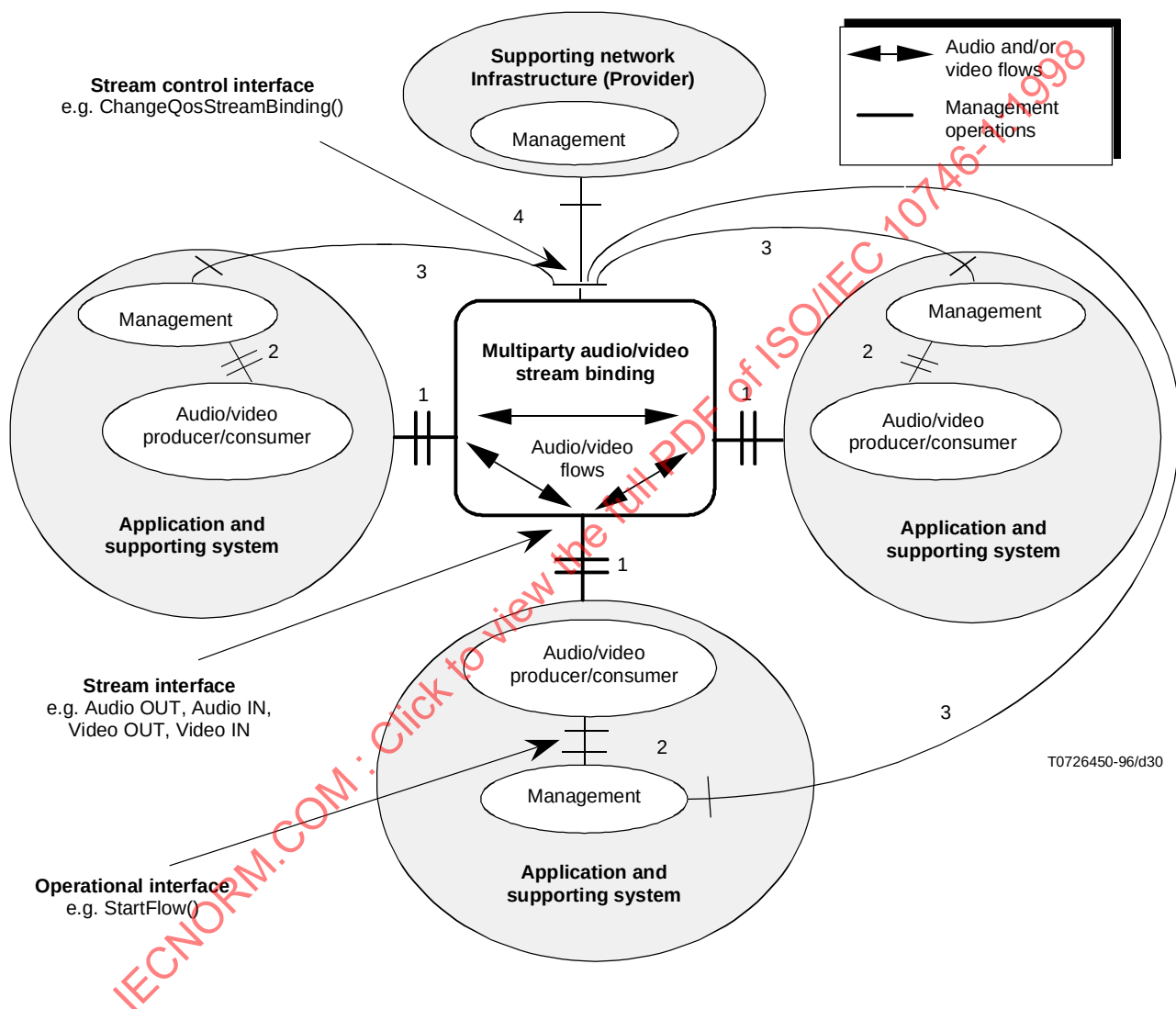
Figure 30 – Multiparty audio/video stream binding
