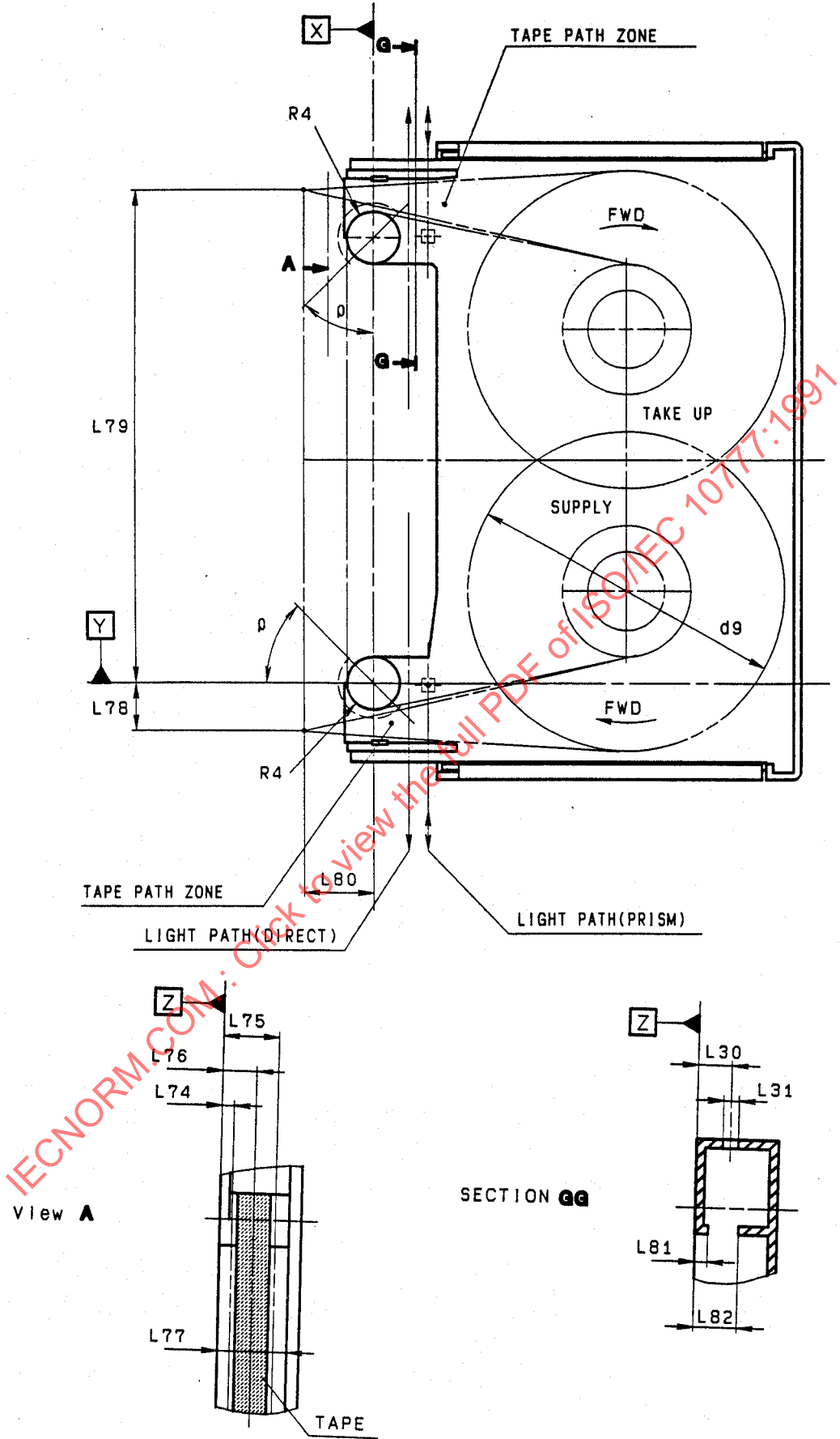
Figure 12 - Inside view of the lower half
