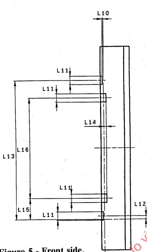
Figure 5 - Front side, lid closed
