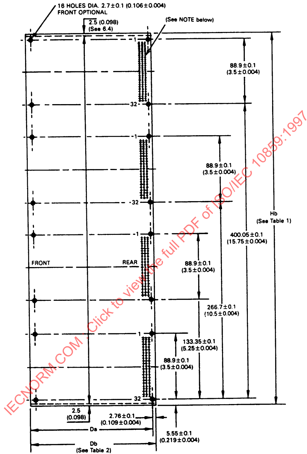
Figure 6 – Quadruple height board, component side view
