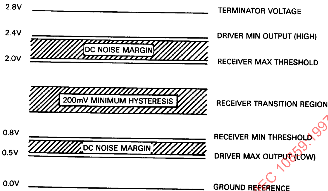
Figure 15 – Signal voltage levels
