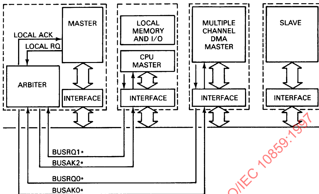
Figure 5 – Example of multiple master implementation
