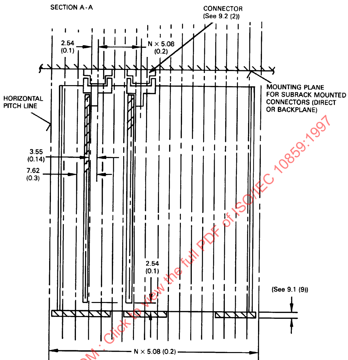
Figure 22 – Box/board type plug-in unit, plan view section A-A
