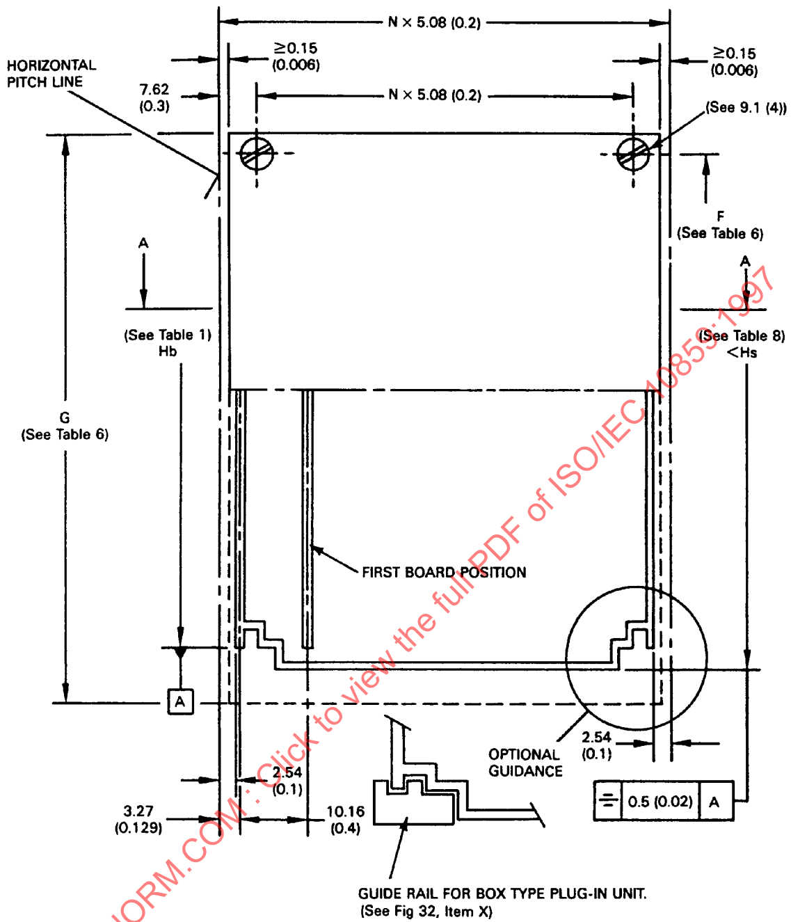
Figure 19 – Box type plug-in unit, front view
