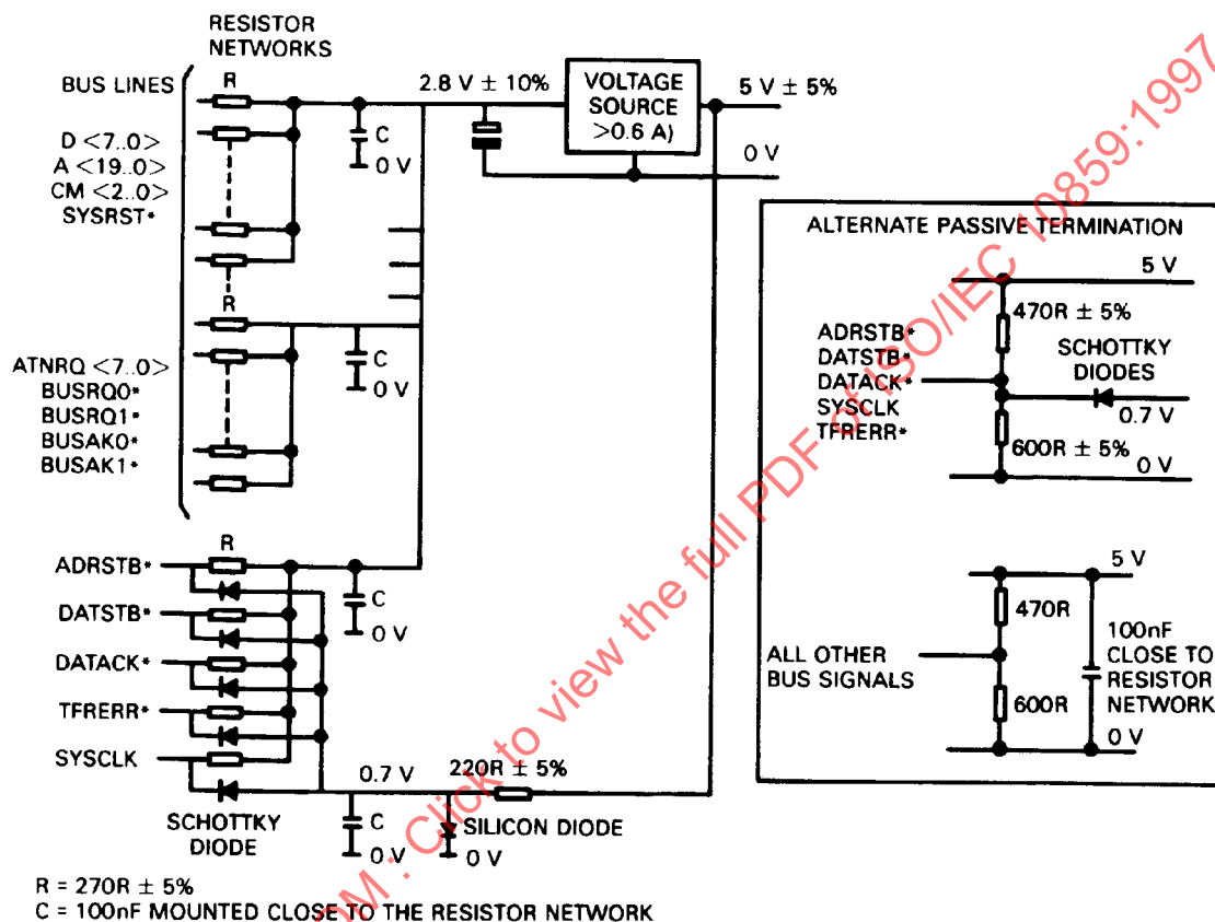
Figure B.1 – Bus termination arrangement
