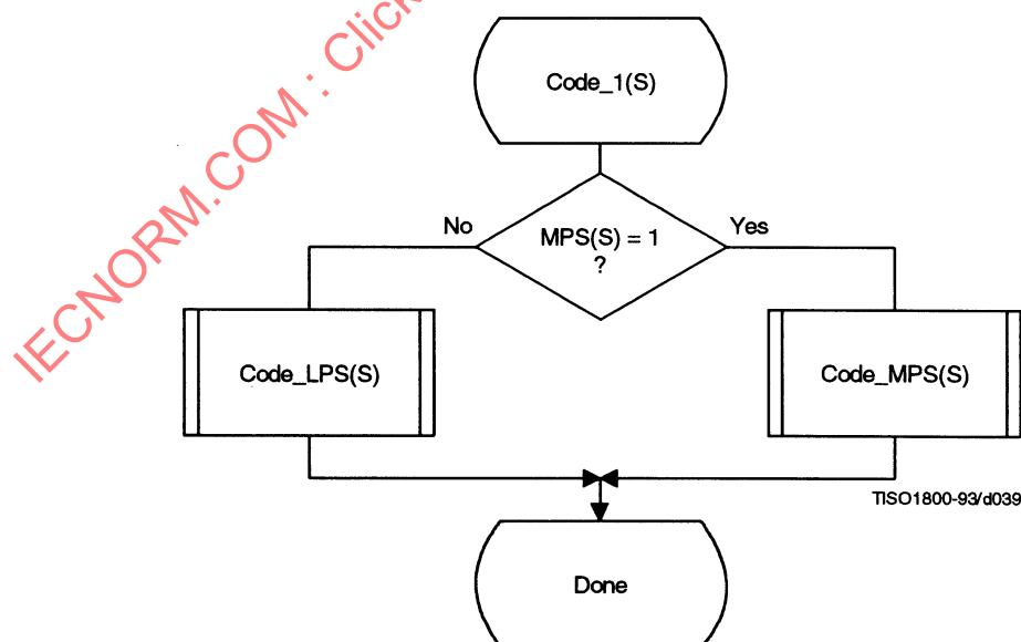
Figure D.1 – Code_1(S) procedure
