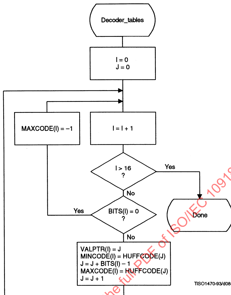
Figure F.15 – Decoder table generation
