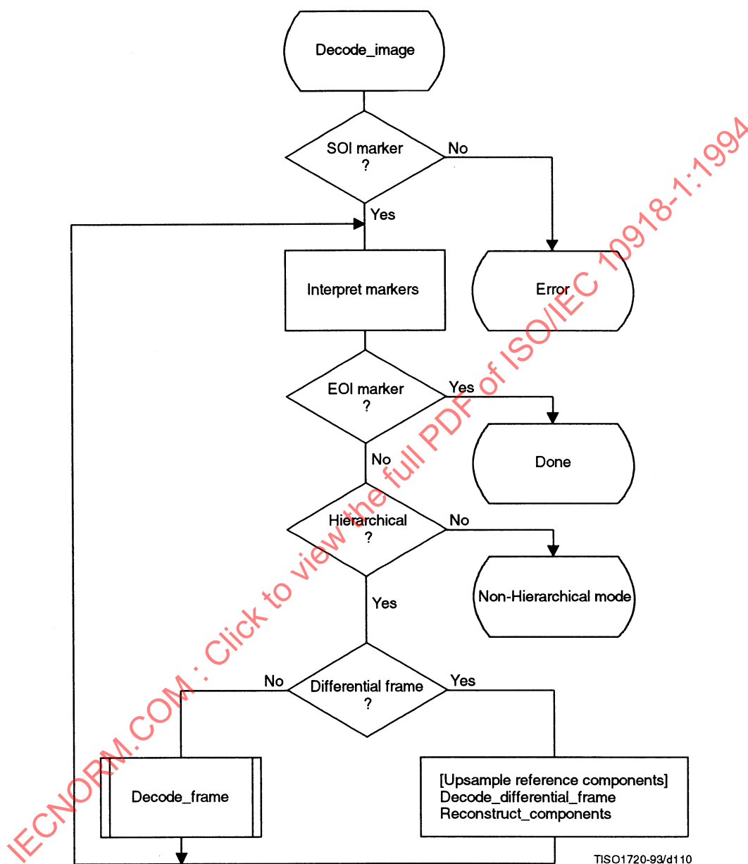
Figure J.3 – Hierarchical control procedure for decoding an image
