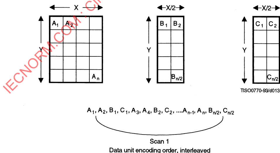
Figure 13 – Interleaved order for components with different dimensions
