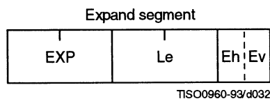
Figure B.14 – Syntax of the expand segment
