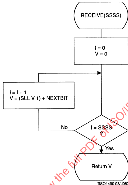
Figure F.17 – Procedure for RECEIVE(SSSS)
