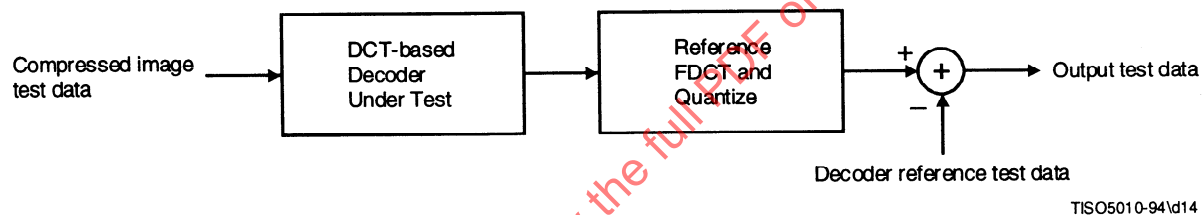
Figure A.2 – Testing procedure for a DCT-based decoder
