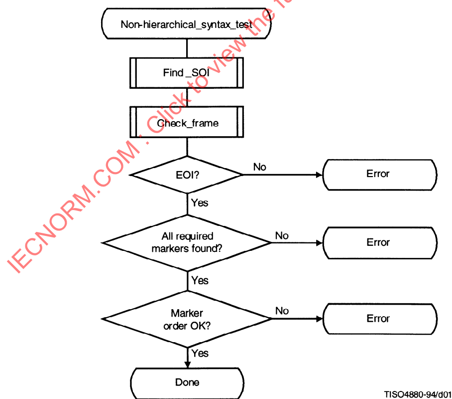
Figure 1 – Non-hierarchical syntax test procedure
