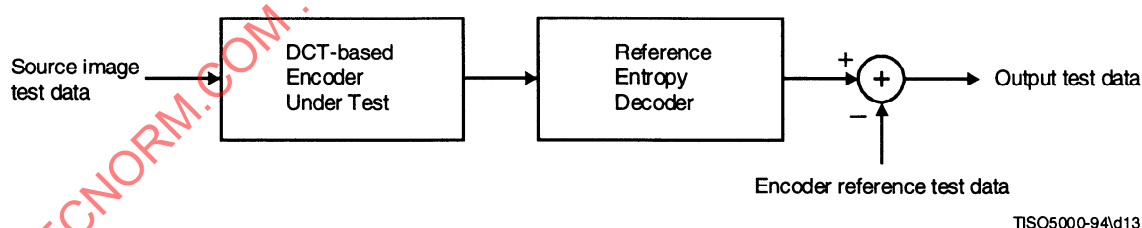
Figure A.1 – Testing procedure for a DCT-based encoder
