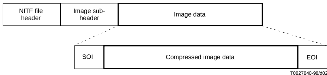
Figure B.1-1 – NITF file structure
