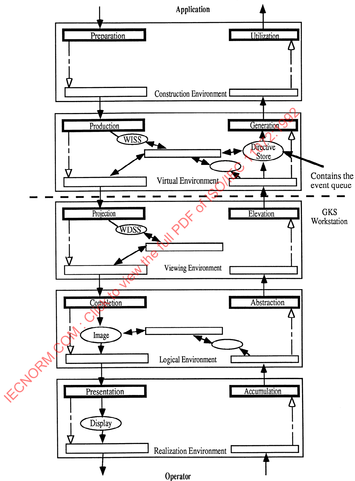
Figure A.1 GKS expressed in terms of the CGRM
