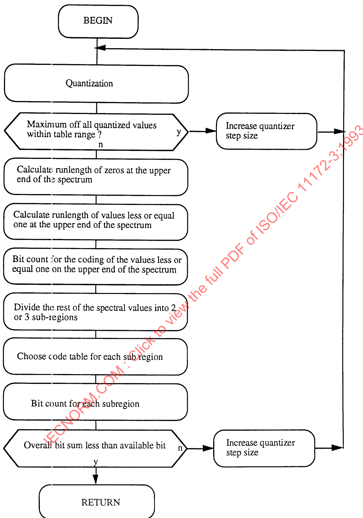
Figure C.9.c -- Layer III inner iteration loop
