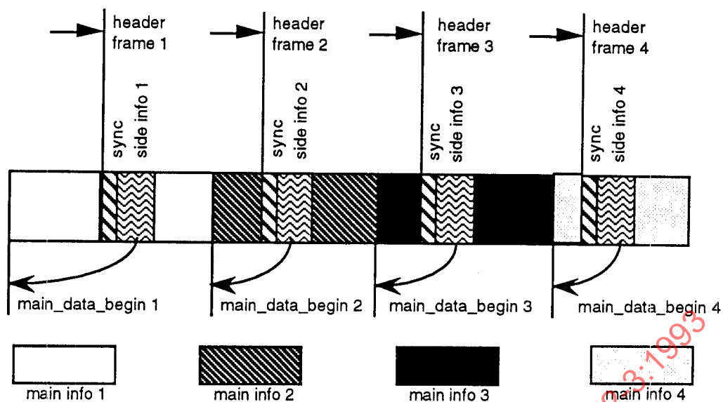
Figure A.7.a -- Layer III bitstream organization
