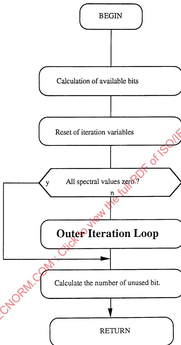
Figure C.9.a -- Layer III iteration loop
