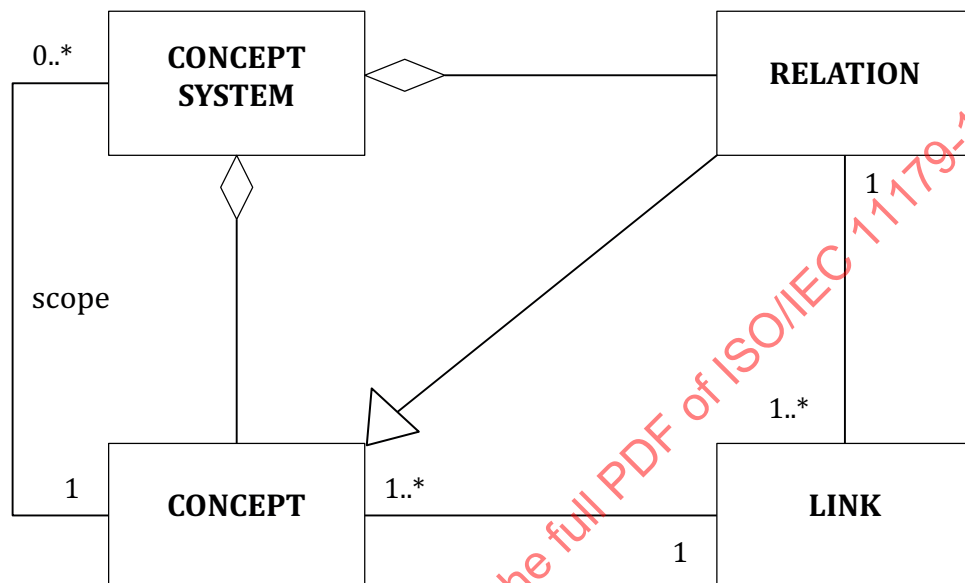
Figure 3 — Fundamental model of concept systems
