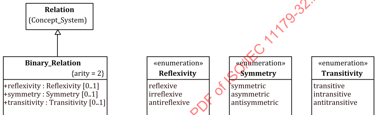
Figure 4 — Binary Relations metamodel region
