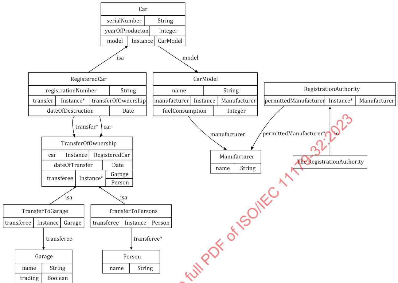
Figure B.2 — Car Registration Ontology in OWL
