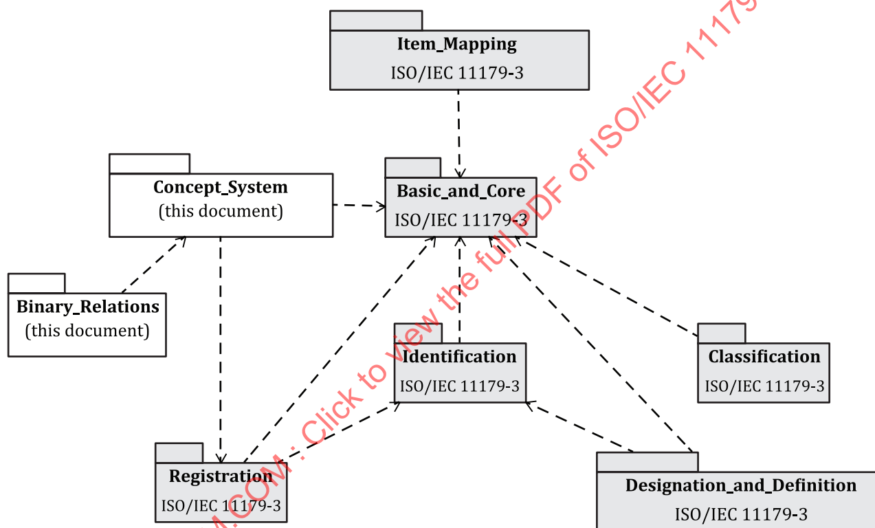
Figure 1 — Package dependencies
