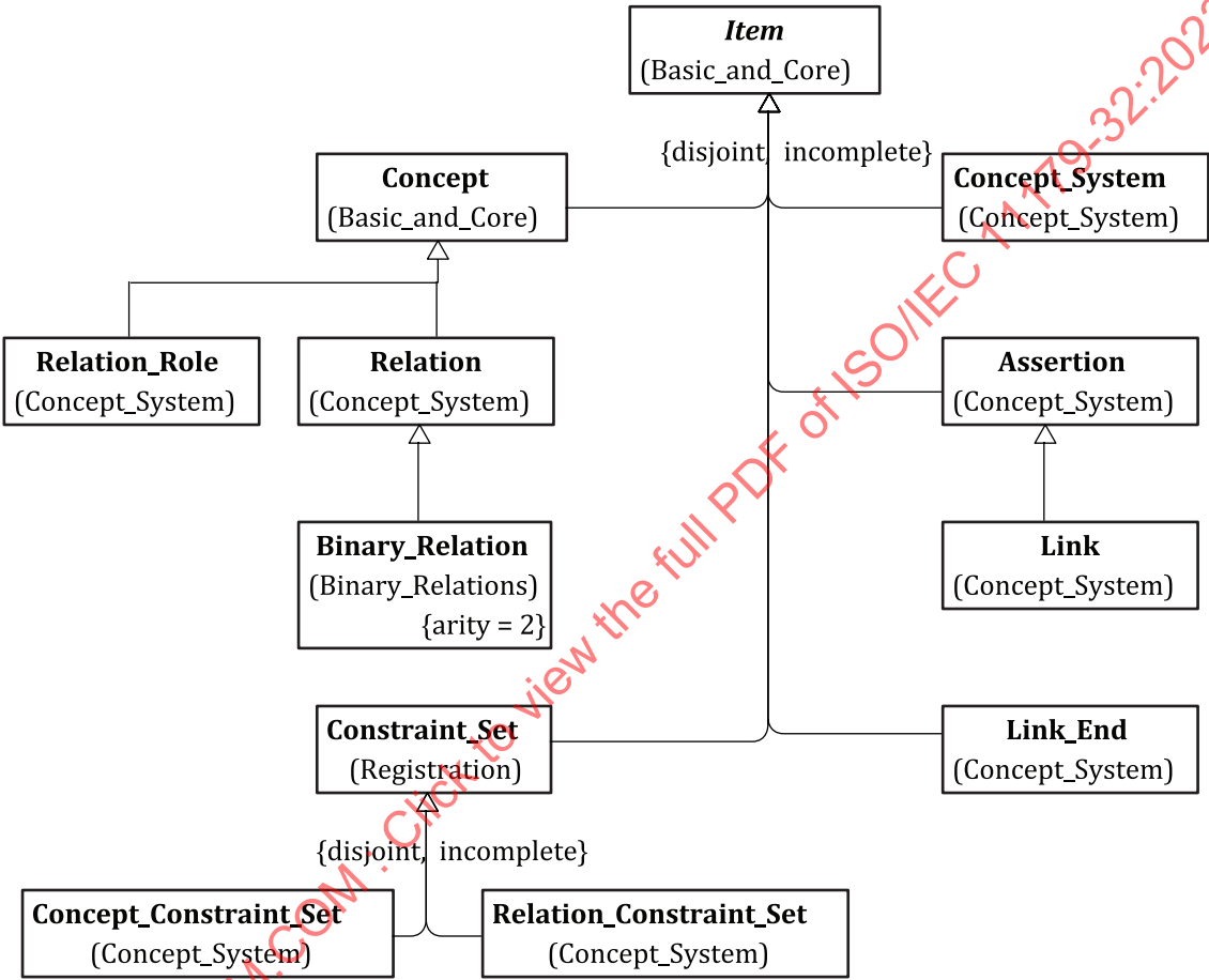
Figure A.1 — Consolidated Class Hierarchy
