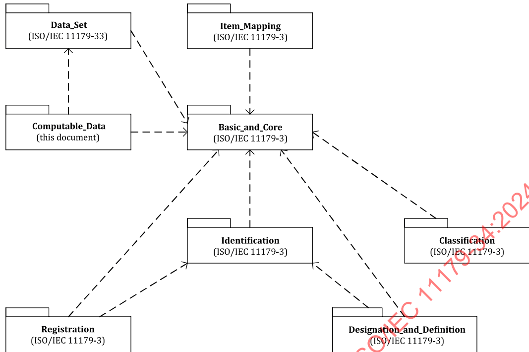
Figure 1 — Package dependencies
