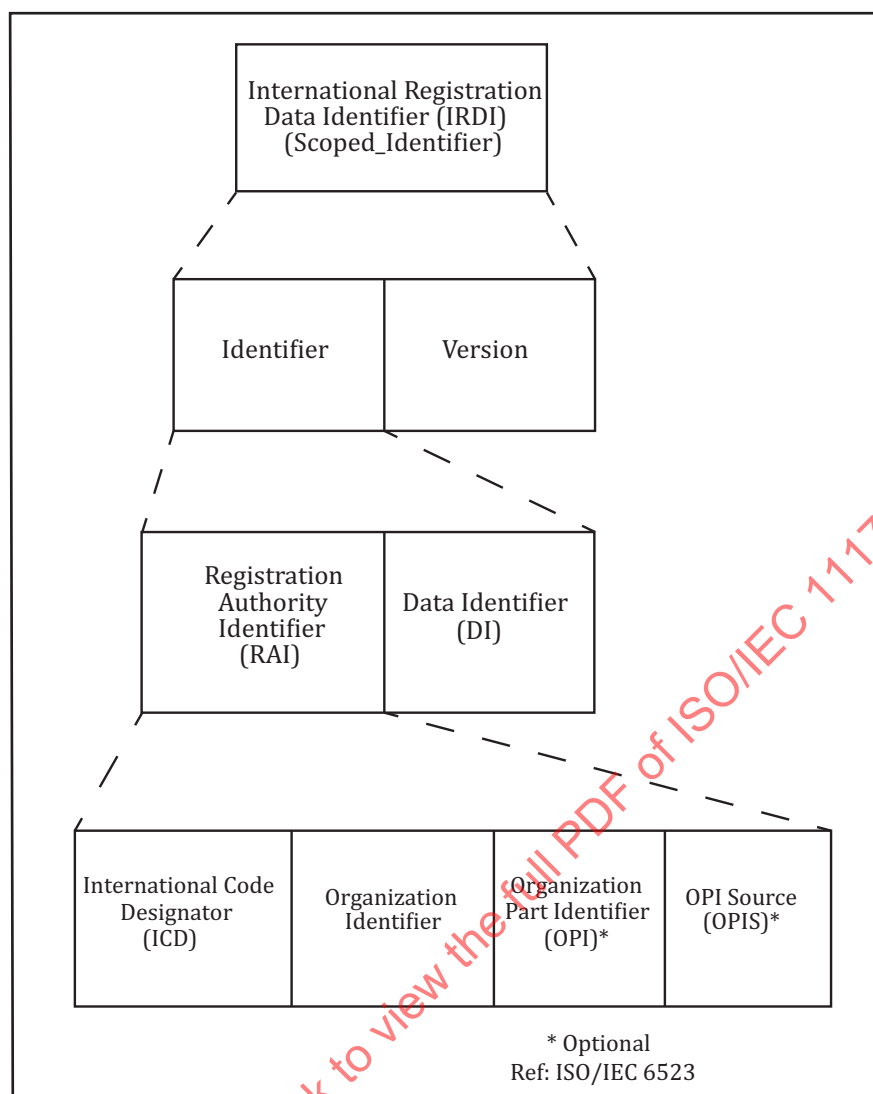
Figure A.1 — Structure of International Registration Data Identifier (IRDI)
