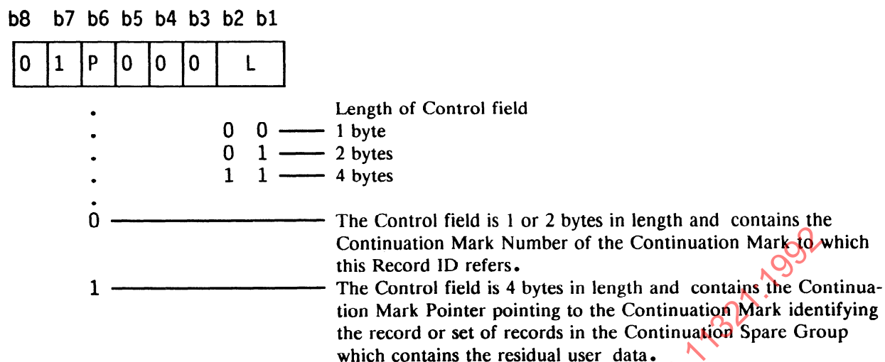
Figure 53 - Control Byte for Continuation Marks
