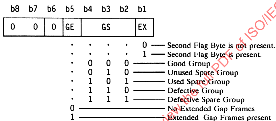
Figure 71 - First Flag Byte for Type A
