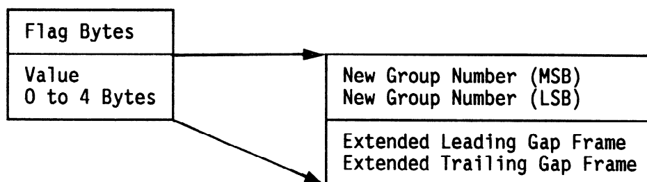
Figure 70 - Type A Group Entry
