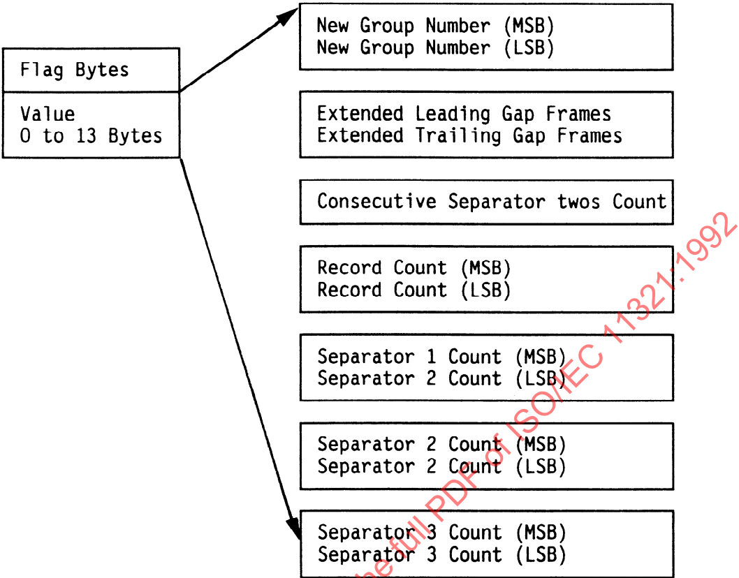
Figure 77 - Type C Group Entry
