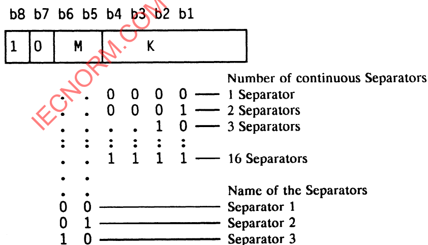
Figure 54 - Control Byte for Separators 1, 2 and 3
