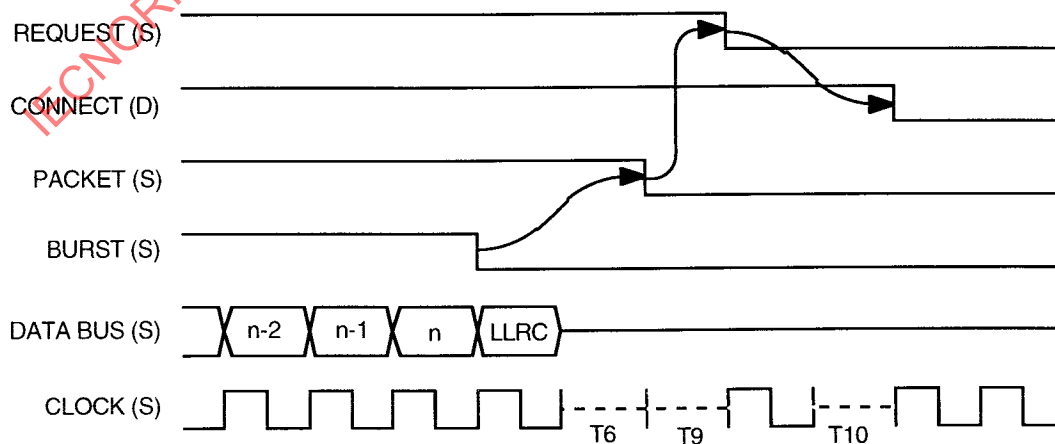
Figure A.5 – End burst, end packet, disconnect
