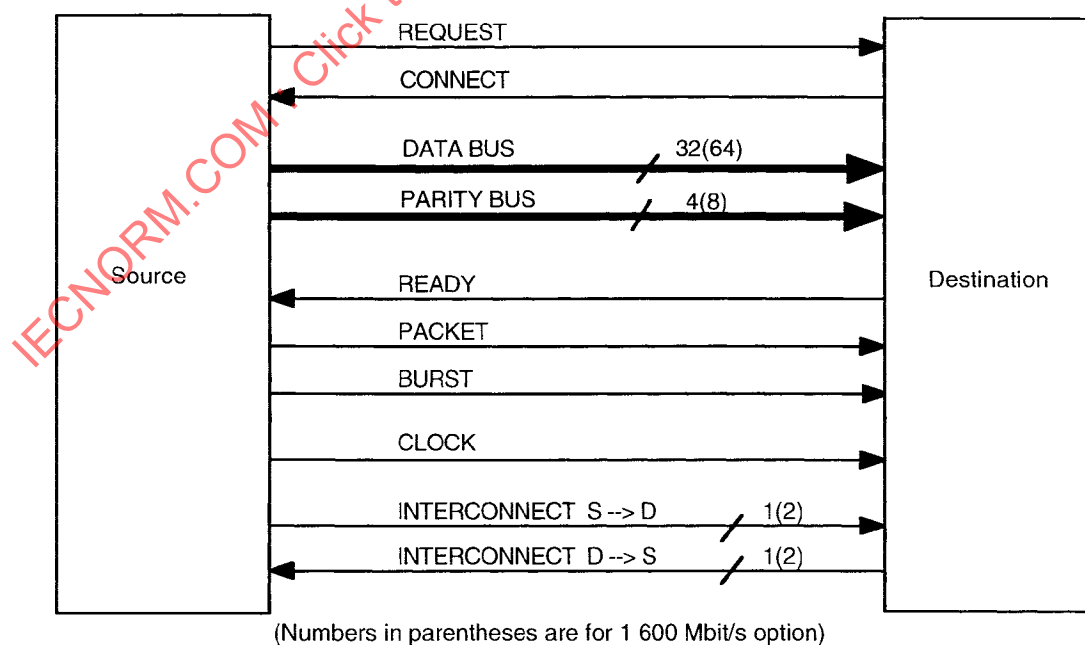
Figure 13 – Interface signal summary
