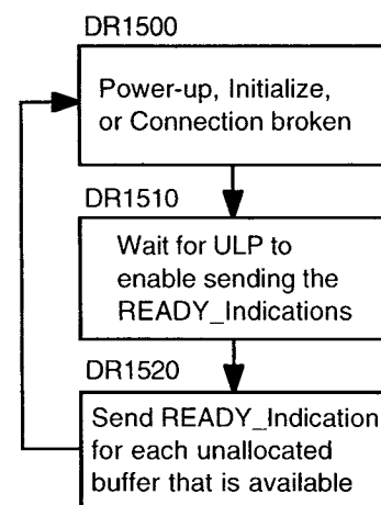
Figure 16 – Destination READY flow diagram
