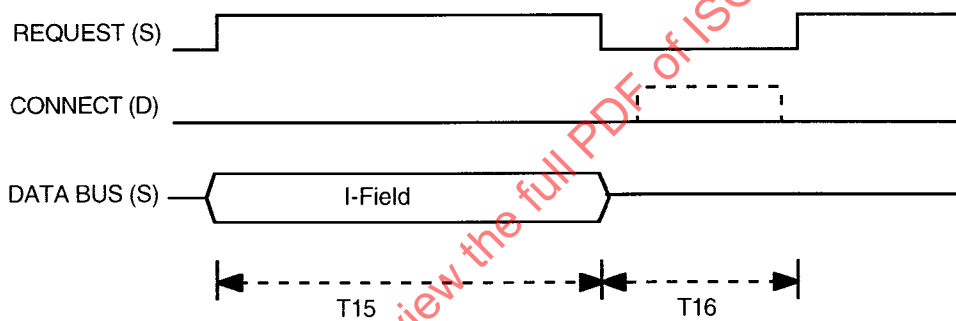
Figure A.8 – Aborted connection sequence
