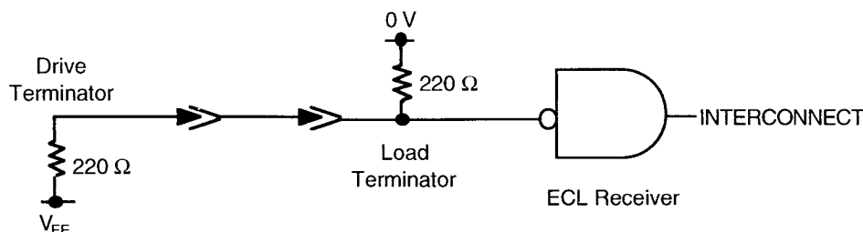
Figure 22 – INTERCONNECT circuit
