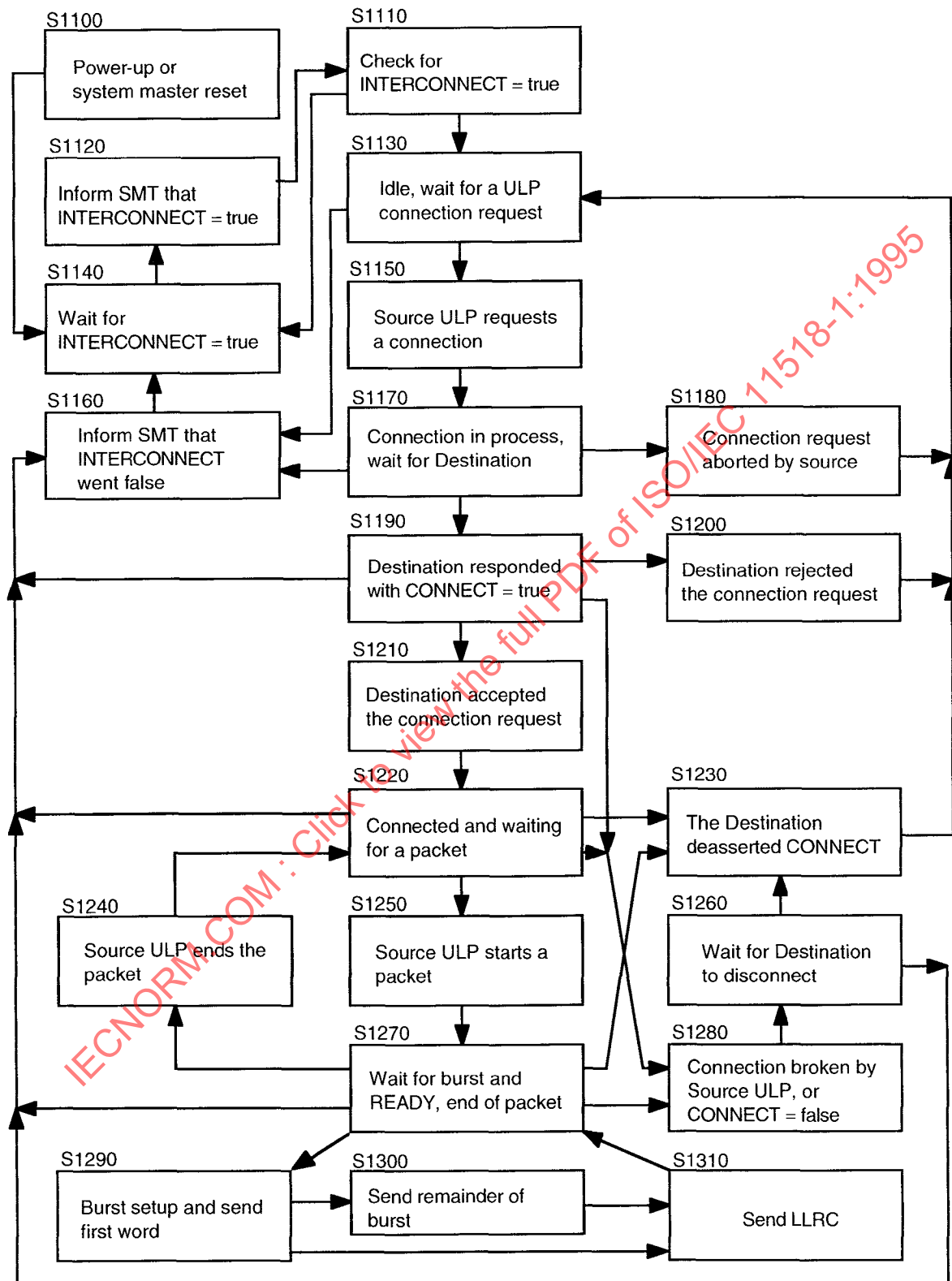
Figure 17 – Source flow diagram
