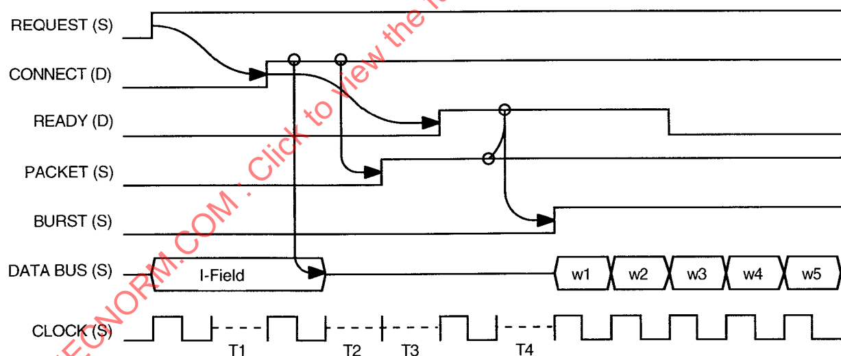
Figure A.2 – Connect, start packet, start burst
