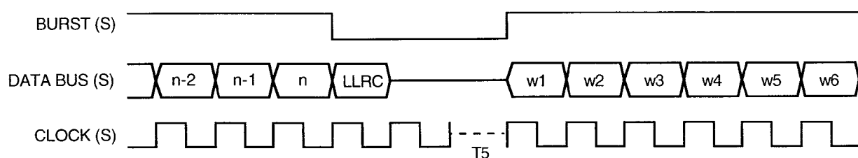
Figure A.3 – End burst, start burst
