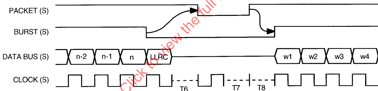
Figure A.4 – End burst, end packet, start packet, start burst
