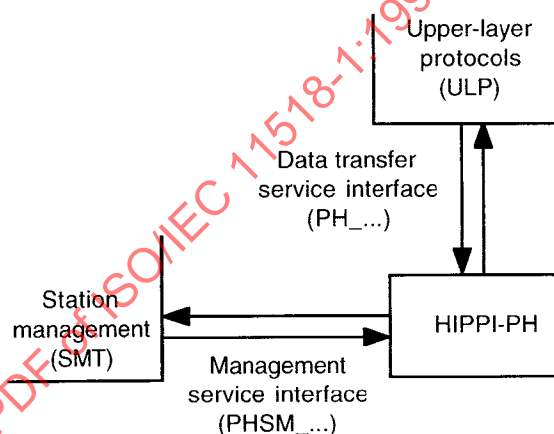
Figure 3 – HIPPI-PH service interface
