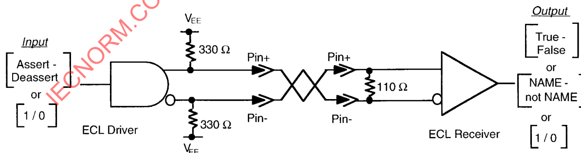
Figure 21 – Differential circuit
