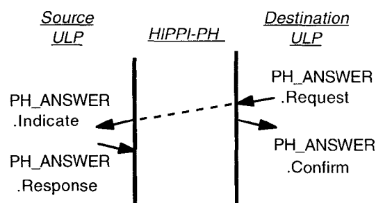
Figure 5 – Complete the connection service primitives
