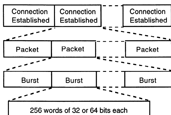
Figure 2 – Logical framing hierarchy
