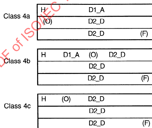
Figure B.4 – Class 4, full burst(s)
