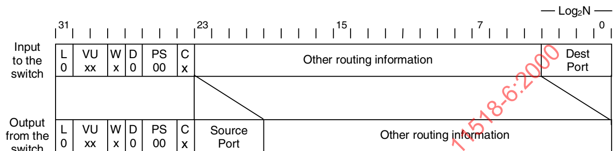
Figure 2 – I-Field with source routing, D = 0, and 16 by 16 switch
