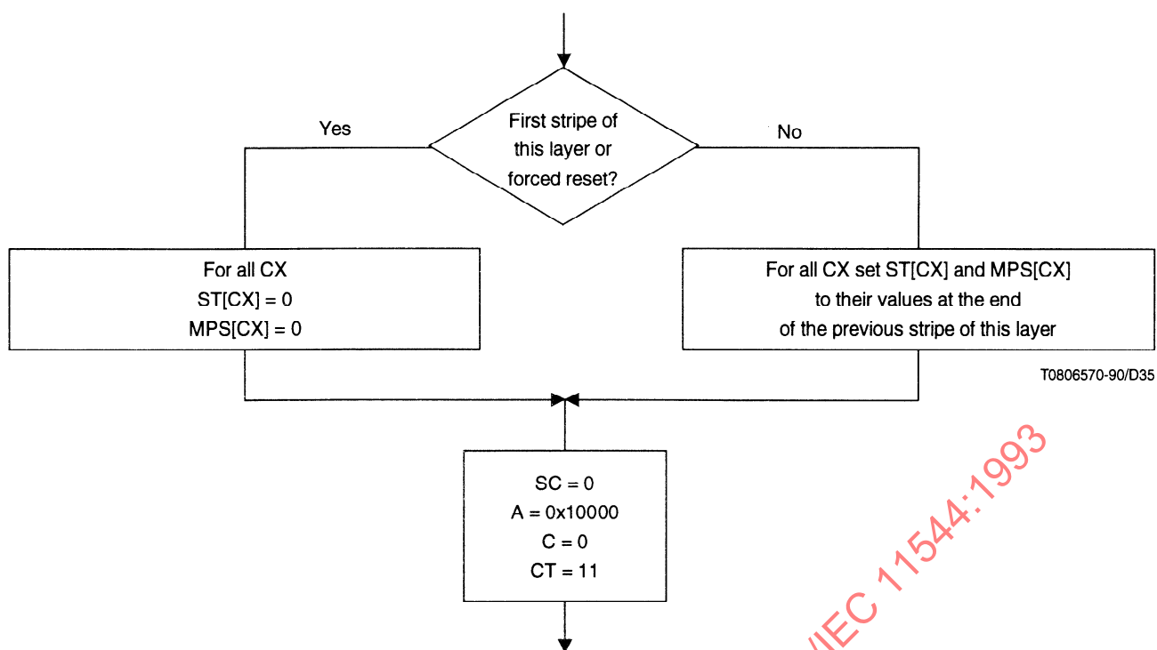
Figure 27 – Flow diagram for the procedure INITENC
