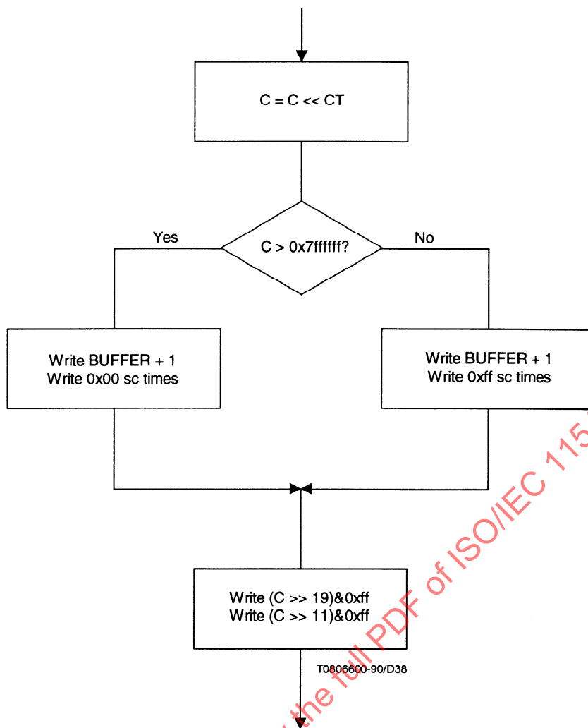
Figure 30 – Flow diagram for the procedure FINALWRITES
