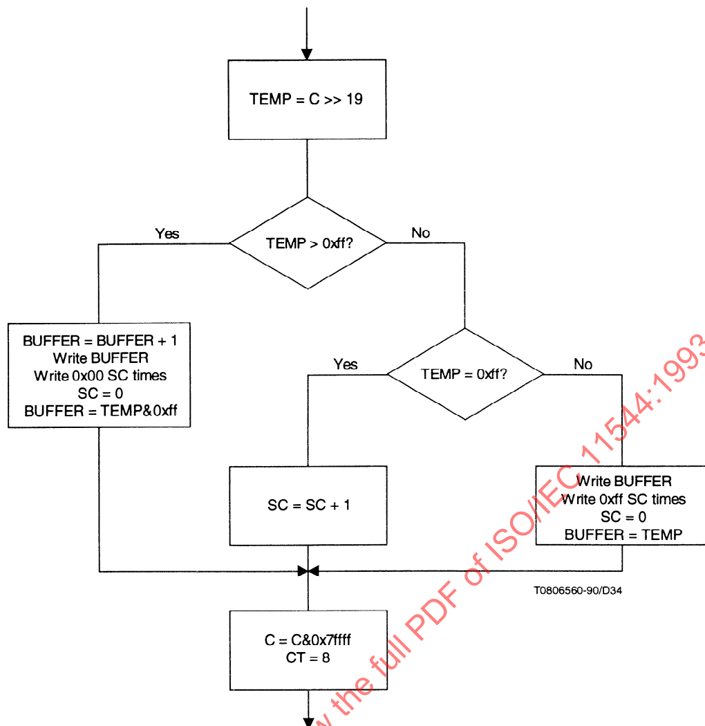
Figure 26 – Flow diagram for the procedure BYTEOUT
