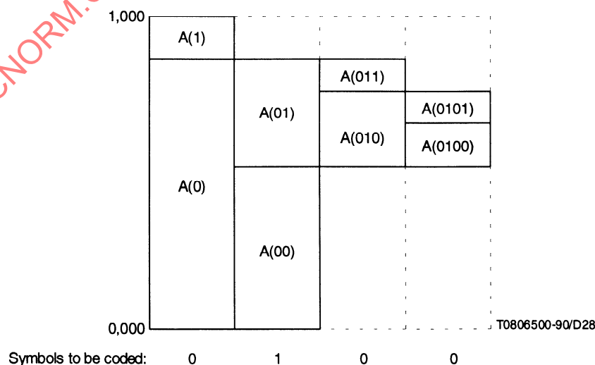
Figure 20 – Interval subdivision
