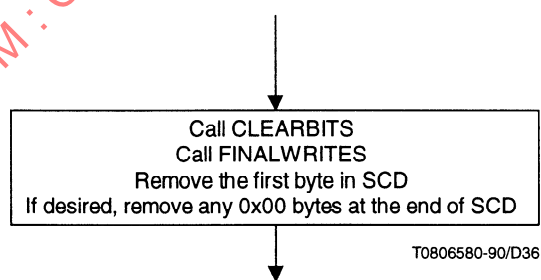
Figure 28 – Flow diagram for the procedure FLUSH
