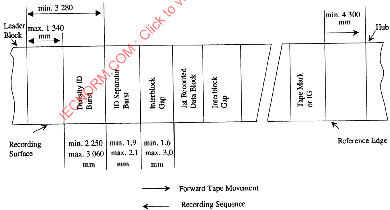
Figure 30 - Arrangement of recording on the tape
