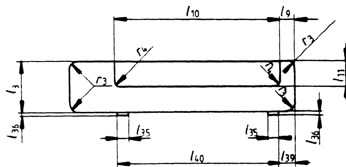
Figure 5 - Rear side of case
