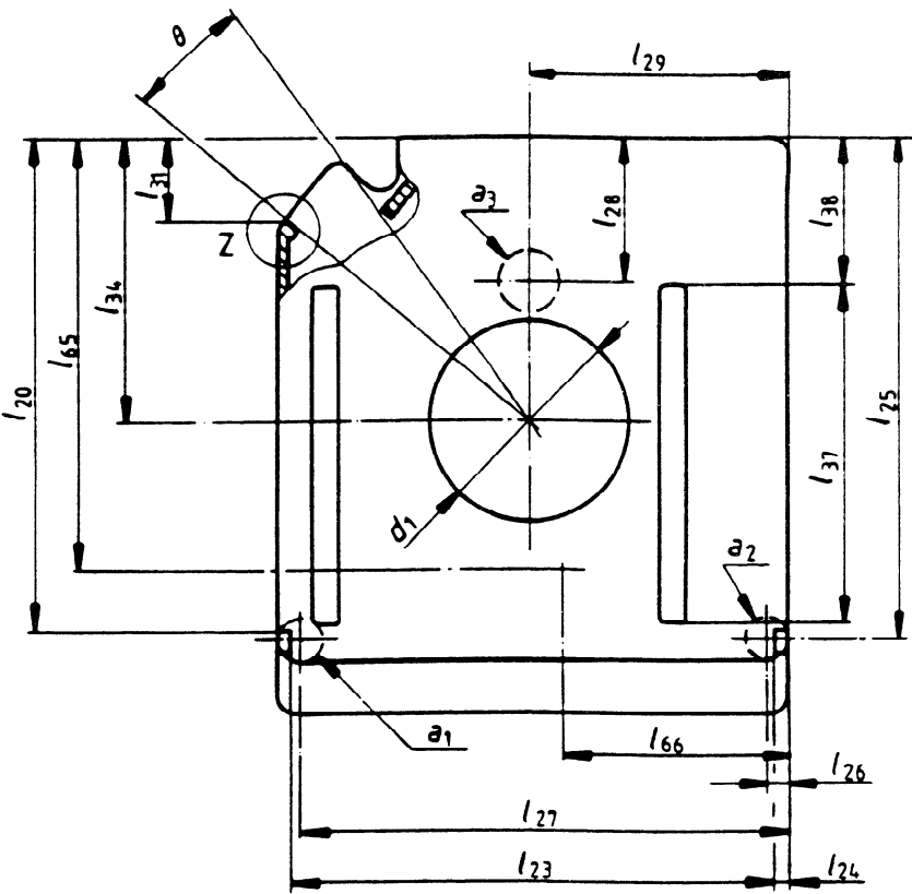
Figure 6 - Bottom side of case
