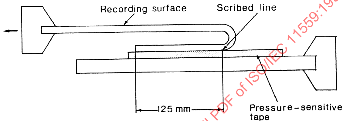
Figure 1 - Coating adhesion
