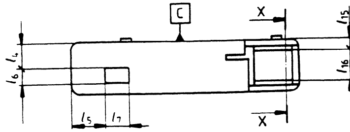
Figure 3 - Front side of case
