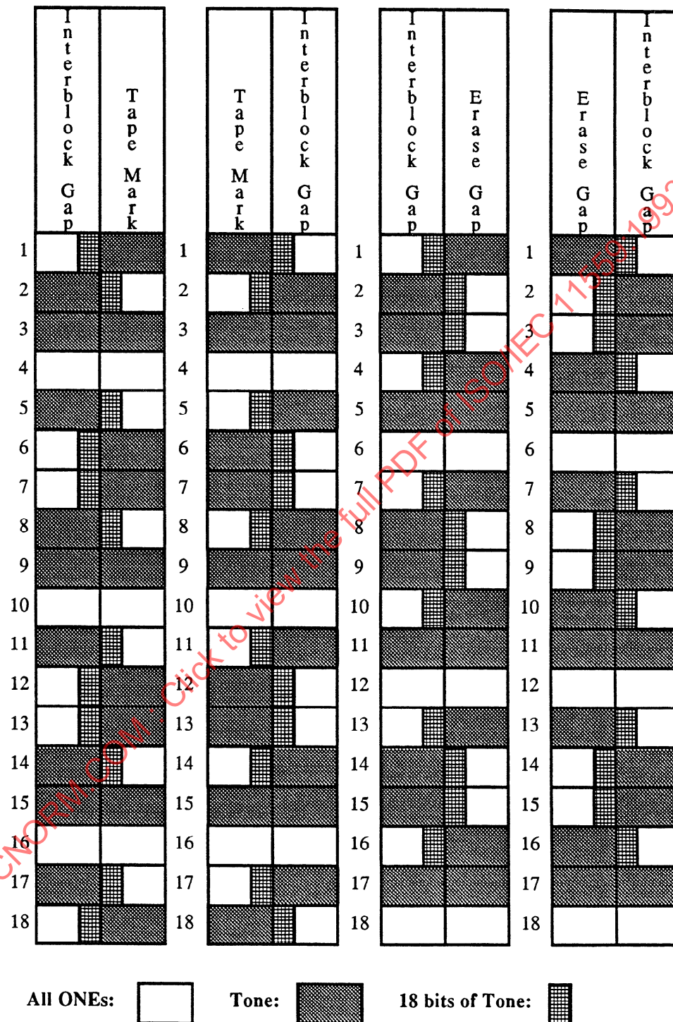
Figure 28 - Relationship between Gaps and Tape Marks
