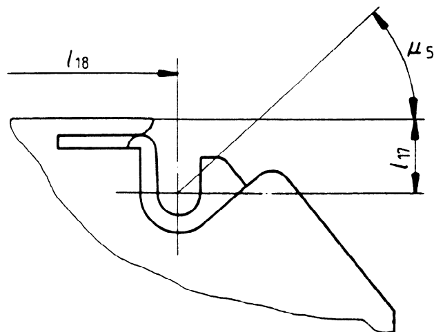
Figure 16 - Leader block in case
