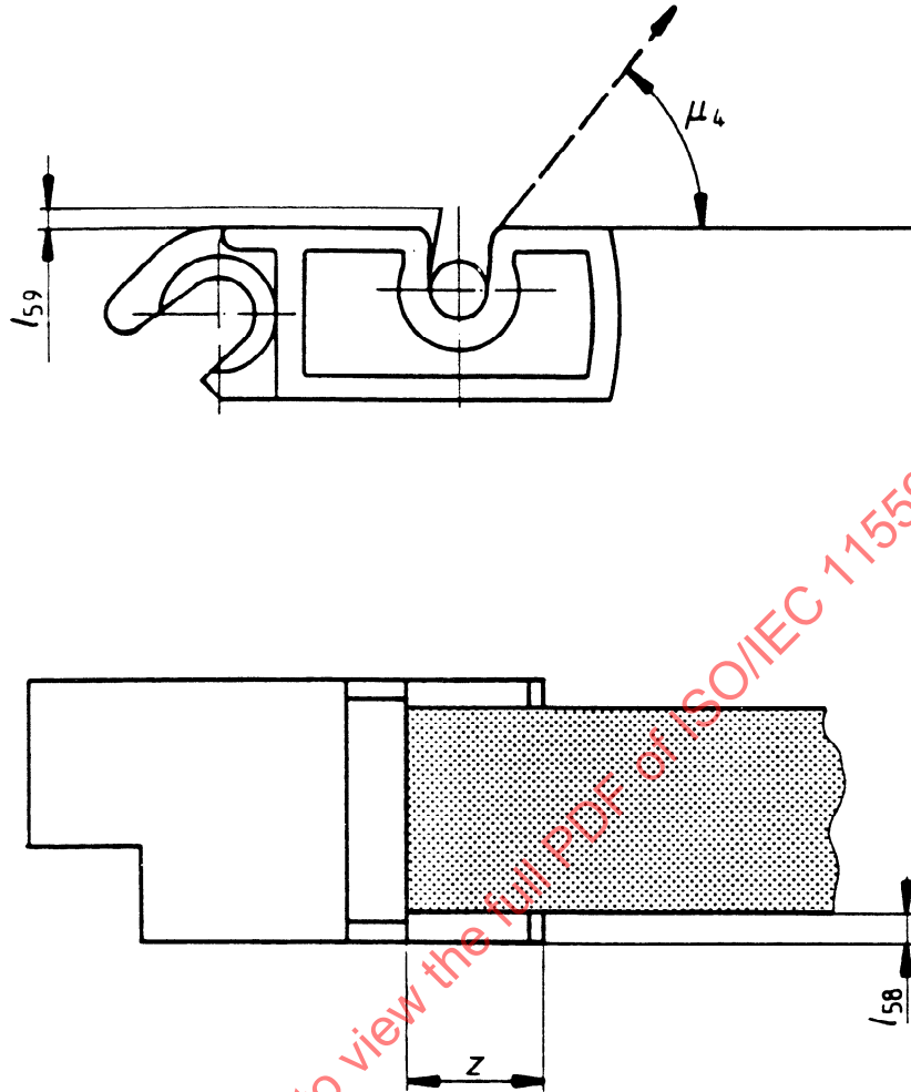
Figure 15 - Fixation of tape to leader block
