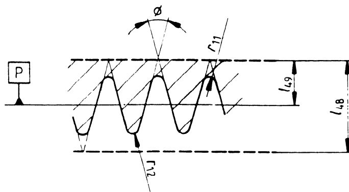
Figure 13 - Teeth of the toothed rim
