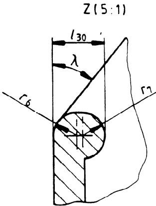
Figure 10 - Cross-section of a detail of the opening of case
