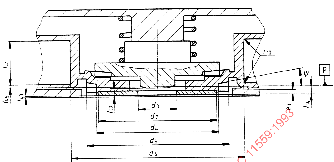
Figure 11 - Cross-section of the cartridge in hand
