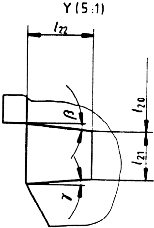
Figure 9 - Cross-section of a location notch
