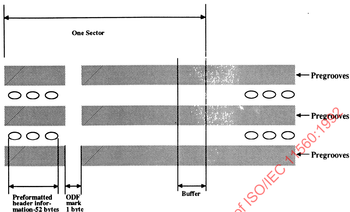
Figure 20 - Example of a sector with Offset Detection Field for on-land recording (schematic)
