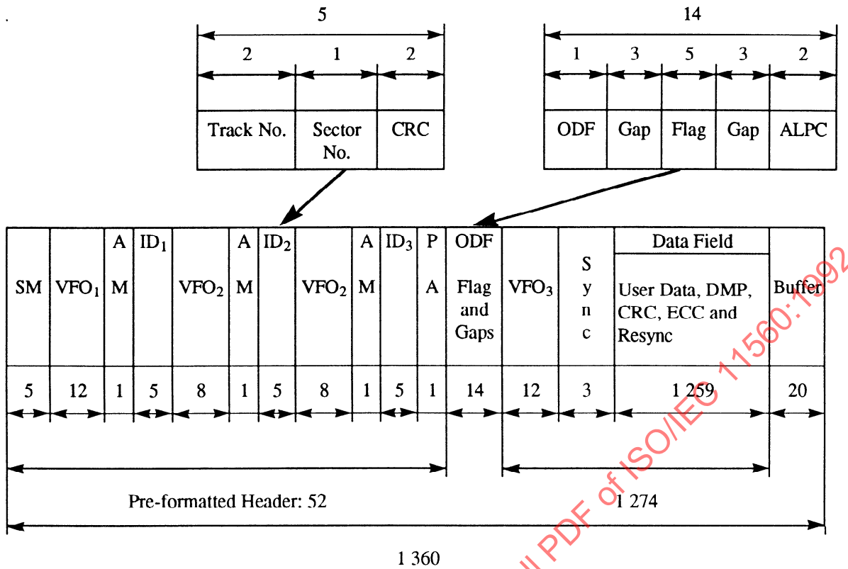
Figure 22 - Sector format for 1 024 user byte
