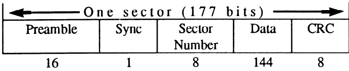
Figure 19 - Sector format in the PEP Zone
