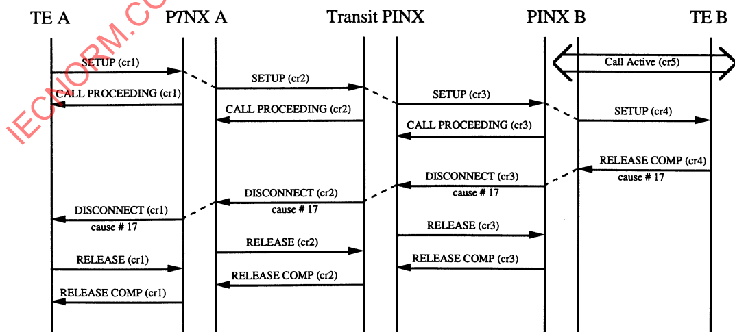
Figure C.2 — Enbloc setup, unsuccessful call
