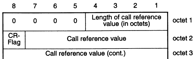
Figure 6 — Call Reference
