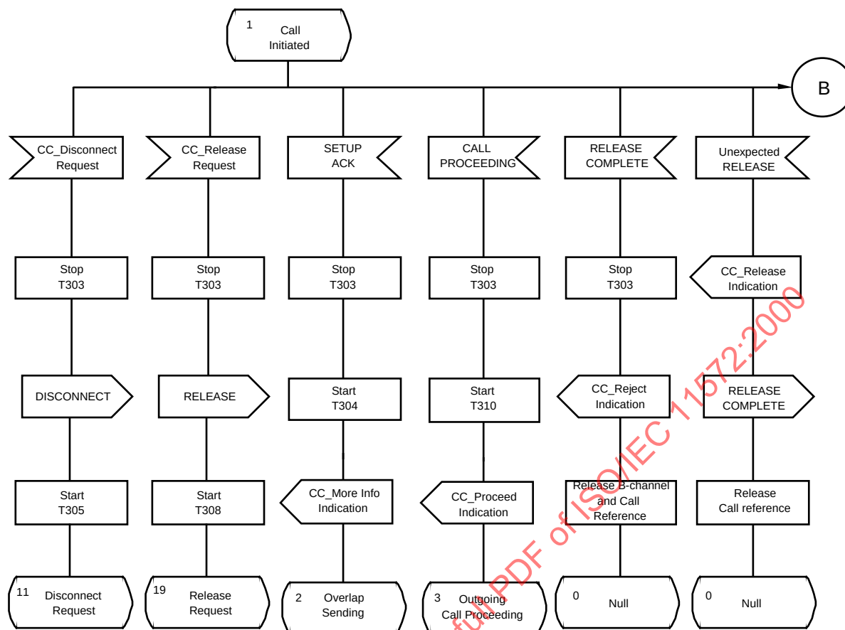
Figure E.2 - Protocol Control SDI diagram (sheet 3 of 22) (continued)
