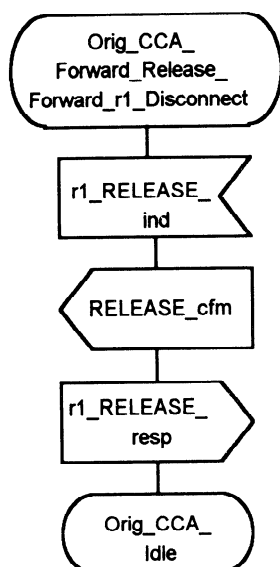
Figure 21 – Stage 2 SDL diagram for Originating CCA functional entity (Sheet 6 of 9)
