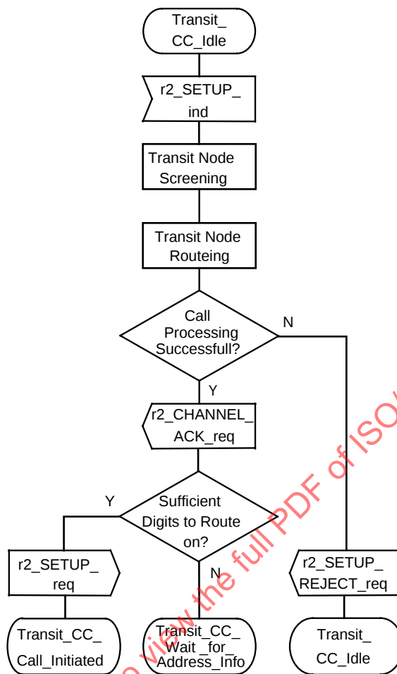
Figure 37 – Stage 2 SDL diagram for Transit CC functional entity (Sheet 1 of 8)
