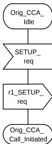
Figure 16 – Stage 2 SDL diagram for Originating CCA functional entity (Sheet 1 of 9)
