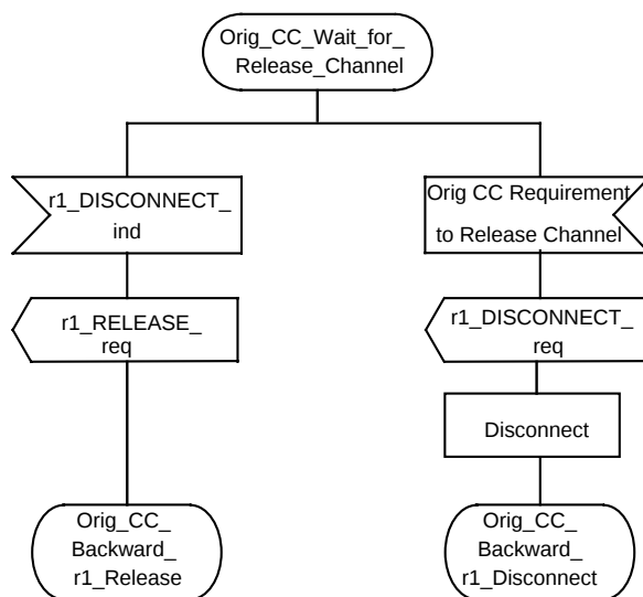
Figure 30 – Stage 2 SDL diagram for Originating CC functional entity (Sheet 6 of 12)
