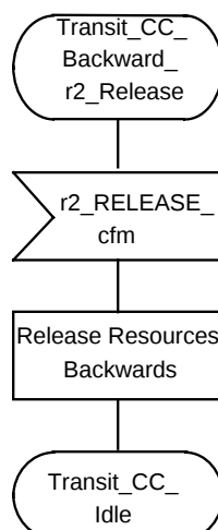
Figure 43 – Stage 2 SDL diagram for Transit CC functional entity (Sheet 7 of 8)
