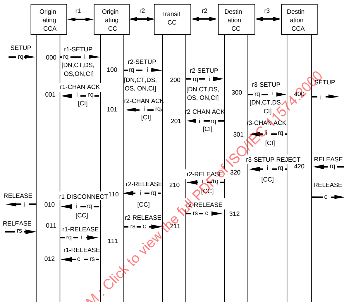
Figure 9 – Unsuccessful calls without the provision of tones and announcements
