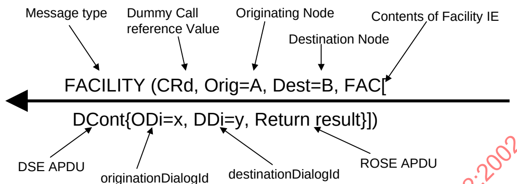
Figure C.10 — Notation for Connectionless Call independent message sequence examples
