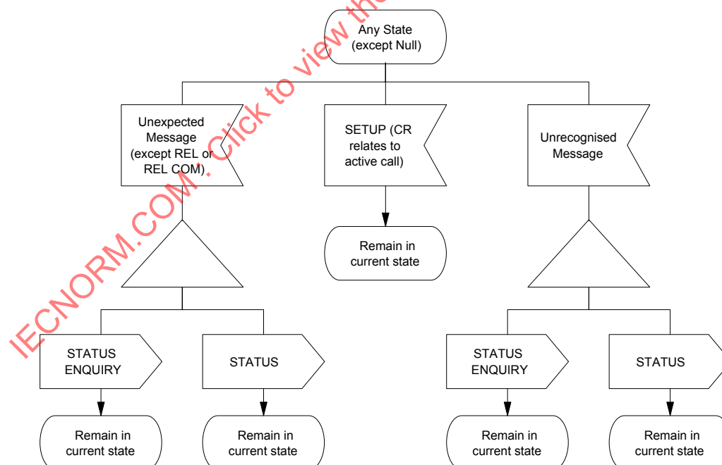
Figure 9 — Connection oriented Protocol Control SDL (Sheet 10 of 10)
