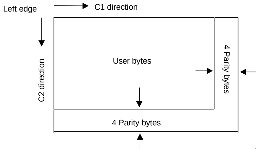
(a) Sector layout with ECC applied
