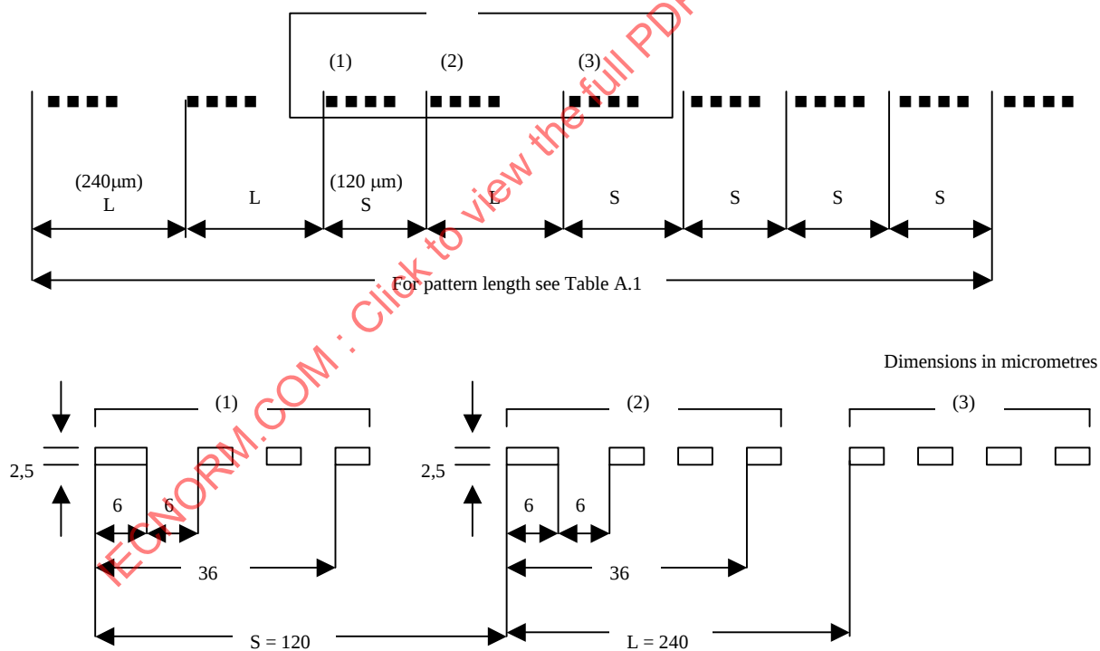
(b) Example of card-type pattern (P11) - See Table A.1
