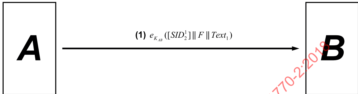
Figure 2 — Mechanism 2
