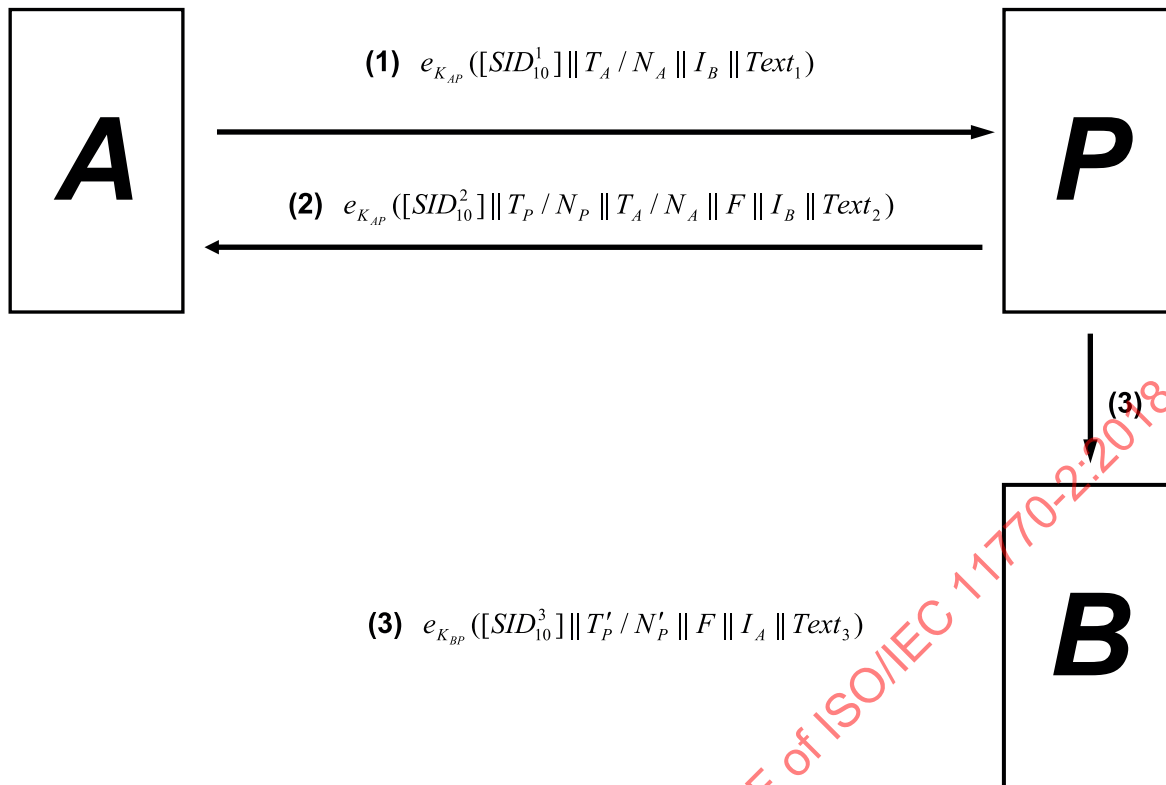
Figure 10 — Mechanism 10
