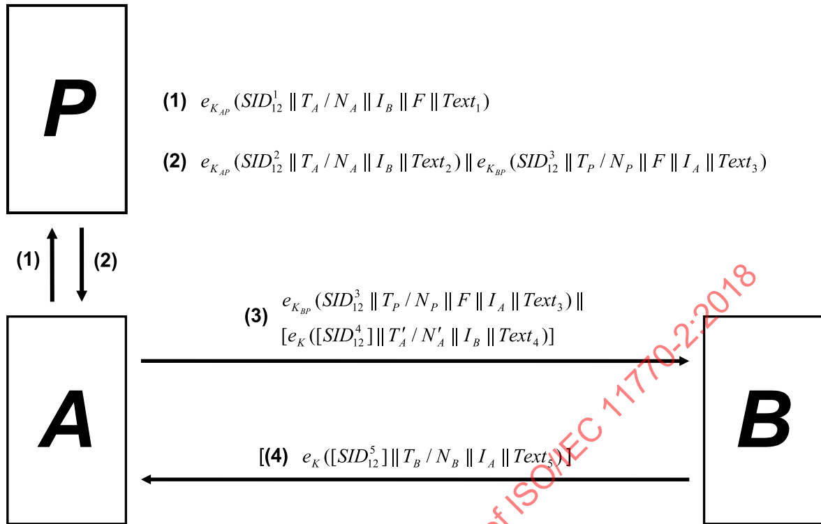
Figure 12 — Mechanism 12
