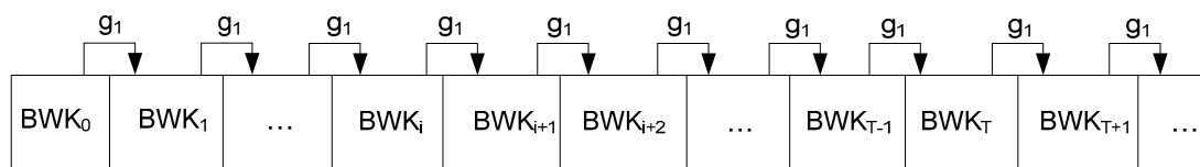
Figure 13 — Calculation of a backward key chain
