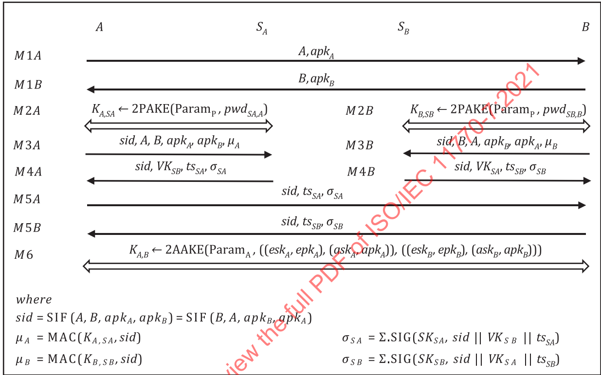
Figure 2 — Mechanism 2
