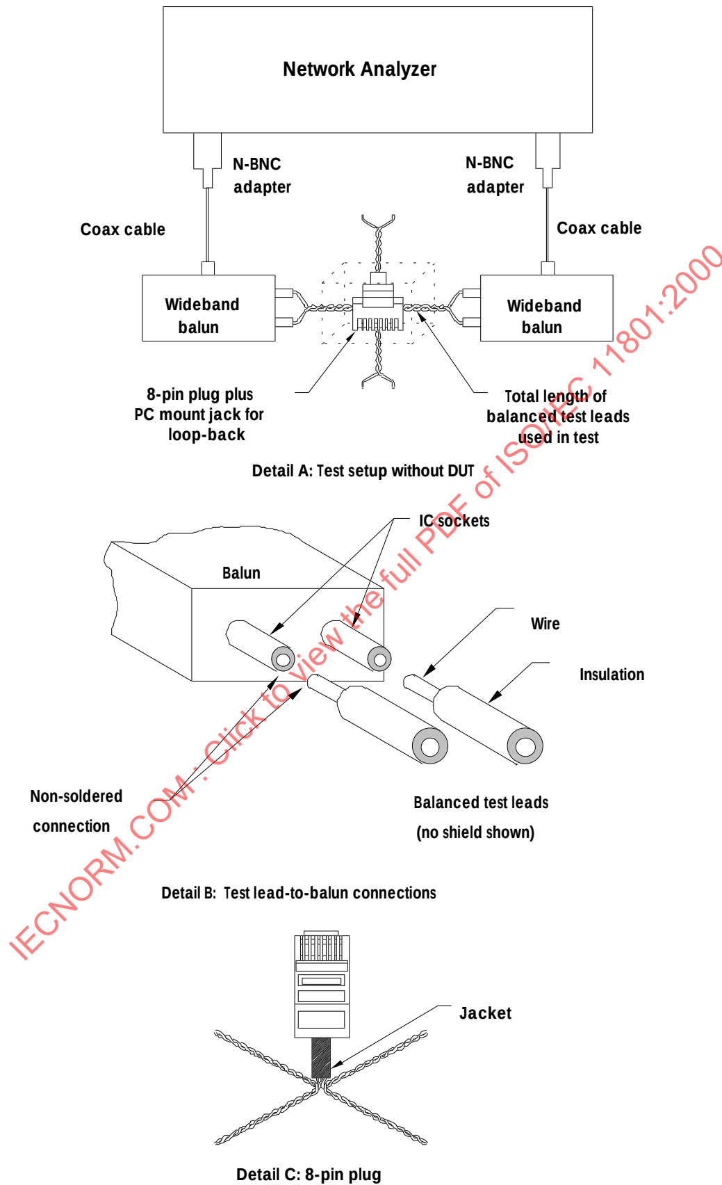
Figure A.11 – Typical TO NEXT measurement set-up
