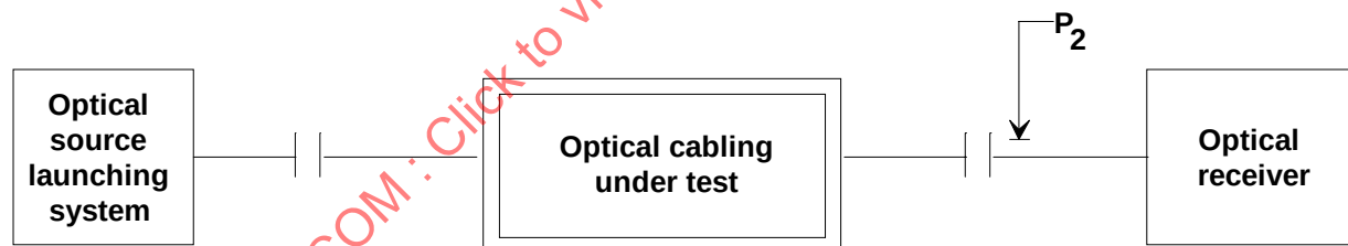
Figure A.4 – Test set-up
