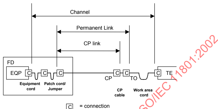
Figure 10 – Channel, permanent link and CP link of a balanced cabling
