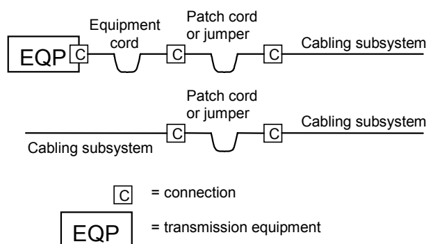
Figure 6 – Cross-connect models
