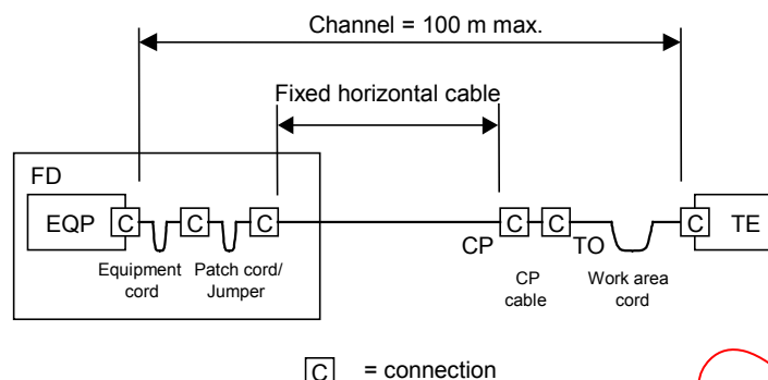
Figure 12 – Horizontal cabling models
